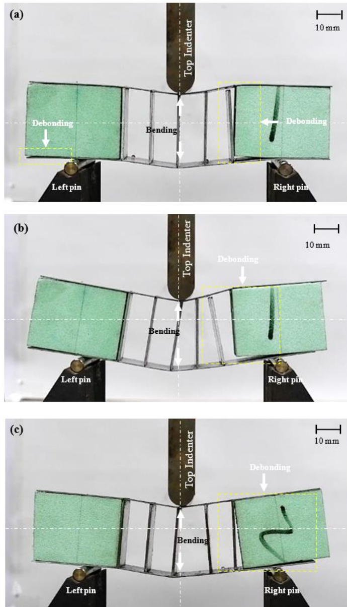
Figure 11. Photographs of damage in five cores with different spacing distance, s : (a,b) 18 mm, (c) 19 mm
