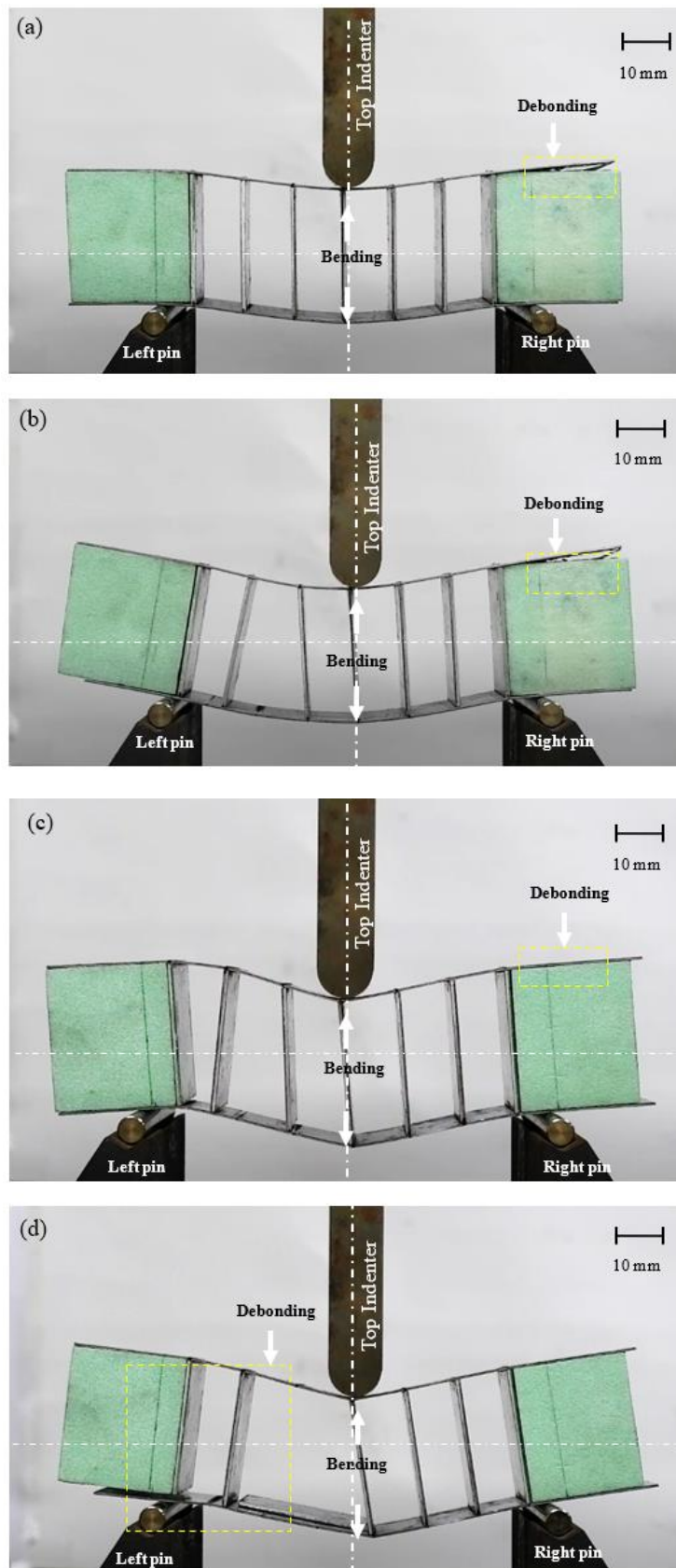
Figure 15. Photographs of failure development in seven cores with different spacing distances, s : (a,b) 18mm, (c,d) 19 mm
