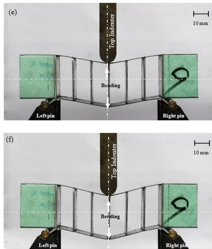
Figure 15. Photographs of failure development in seven cores with different spacing distances, s : (e,f) 20 mm (cont.)
