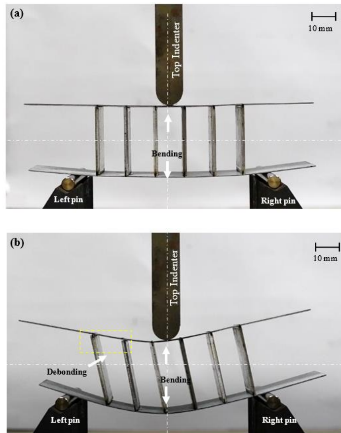
Figure 9. (a) and (b) Photographs of damage development in 6 cores with spacing distance, s = 19 mm
