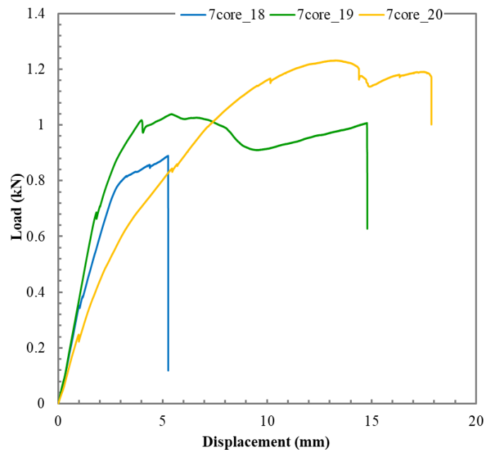
Figure 14. Load-displacement trace on three-point bending test of seven cores with different spacing distances, s = 18 , 19, and 20 mm
