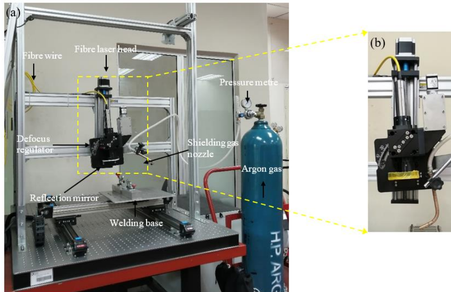
Figure 6. (a) Laser welding setup with complete installation equipment of welding process, (b) close-up of fibre laser head
