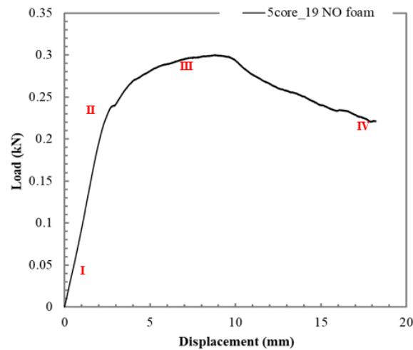
Figure 6. Load-displacement trace on three-point bending test of five cores with spacing distance, s = 19 mm
