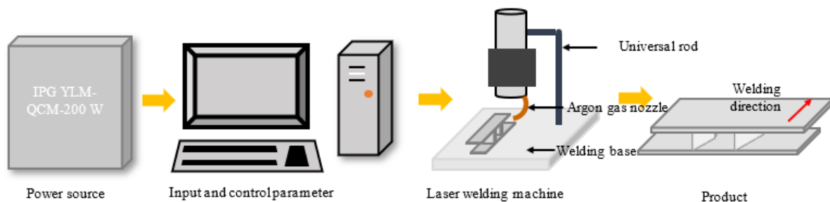
Figure 4. Schematic diagram of laser welding process on web-core sandwich structure
