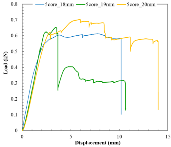
Figure 10. Load-displacement trace on three-point bending test of five cores with different spacing distances, s = 18 , 19, and 20 mm
