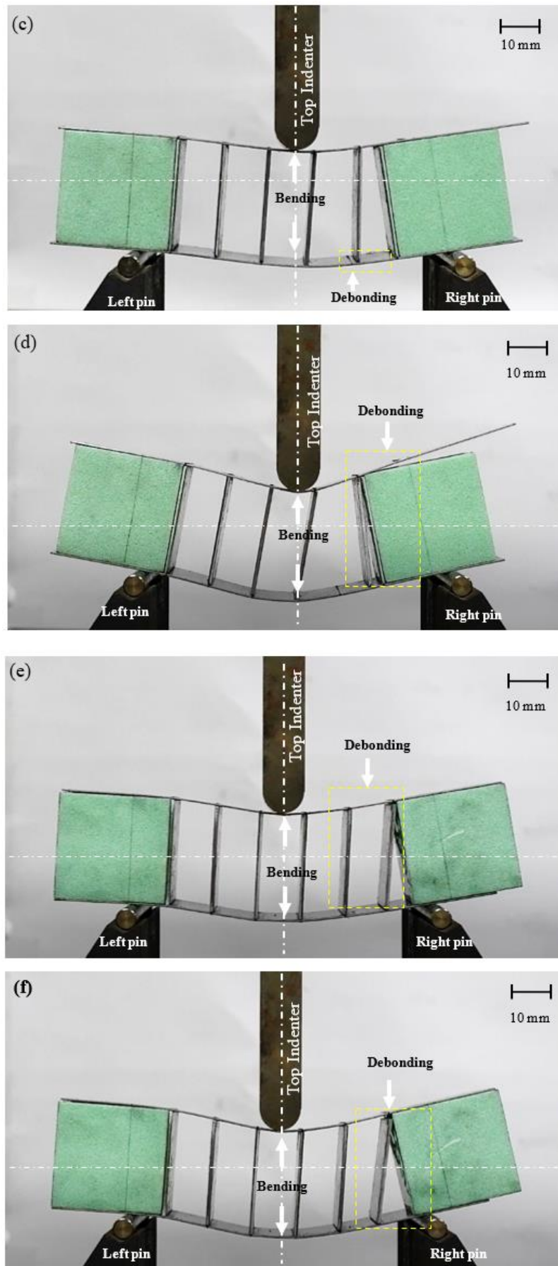
Figure 13. Photographs of damage in six cores with different spacing distance, s : (c,d) 19 mm, and (e,f) 20 mm (cont.)
