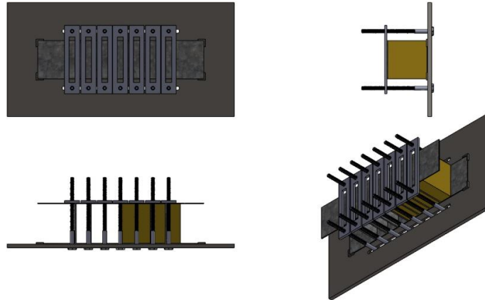
Figure 3. Welding jig to setup a web-core sandwich structure
