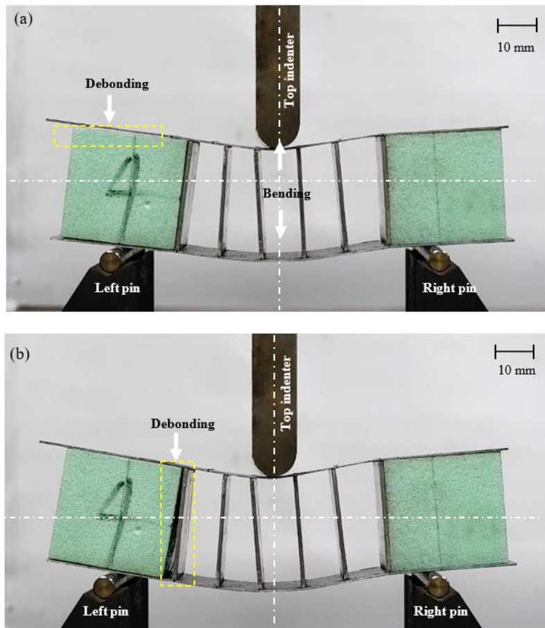
Figure 13. Photographs of damage in six cores with different spacing distance, s : (a,b) 18 mm
