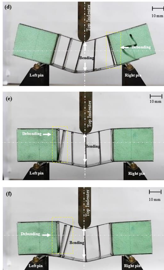
Figure 11. Photographs of damage in five cores with different spacing distance, s : (d) 19 mm, and (e,f) 20 mm (cont.)
