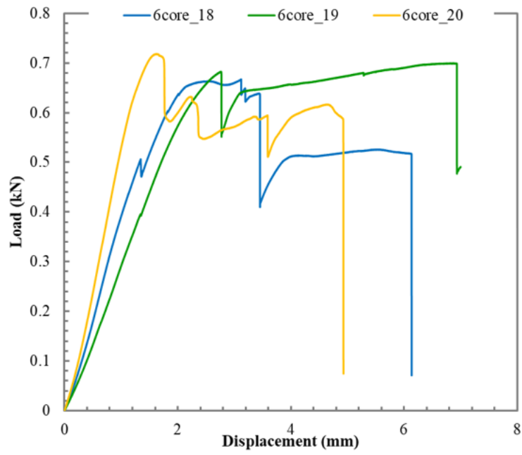
Figure 12. Load-displacement trace on three-point bending test of six cores with different spacing distance, s = 18, 19, and 20 mm
