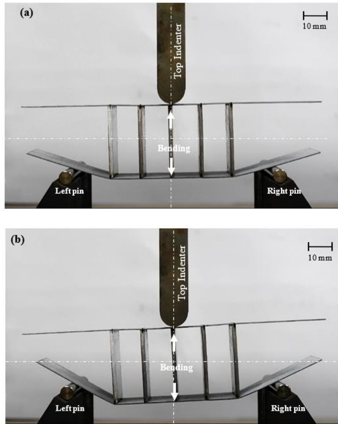
Figure 7. (a) and (b) Photographs of damage development in five cores with spacing distance, s = 19 mm
