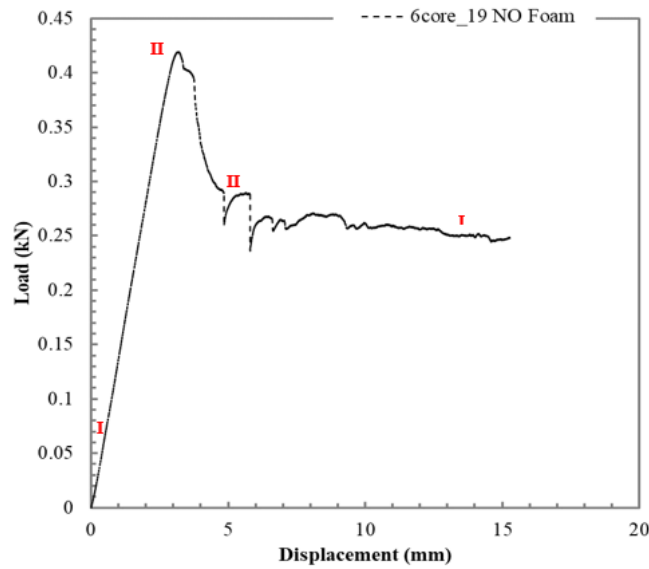
Figure 8. Load-displacement trace on three-point bending test of six cores with spacing distance, s = 19 mm
