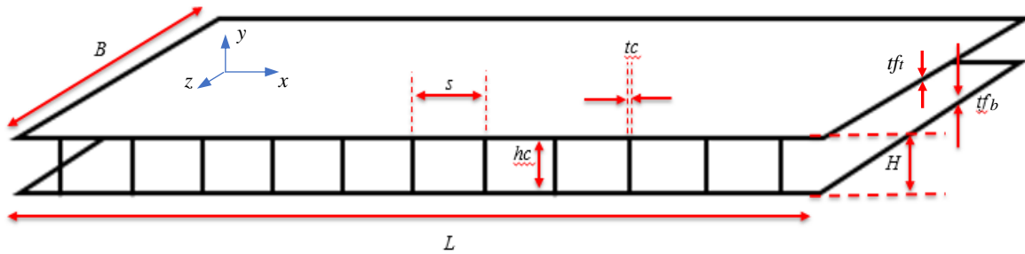
Figure 2. Illustration of web-core sandwich structure
