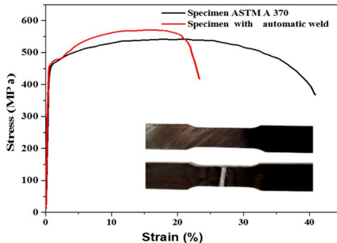
Figure 6. Stress-Strain curve for API X 52 pipeline steel when tested with specimen automatic weld and without weld
