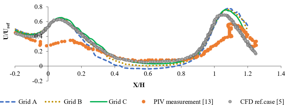
Figure 5. Comparison of the three different cell counts for coarse (Grid A), medium (Grid B) & fine (Grid C) with result of PIV measurement by Karava et al. [13] and numerical results by Ramponi and Blocken [5]
