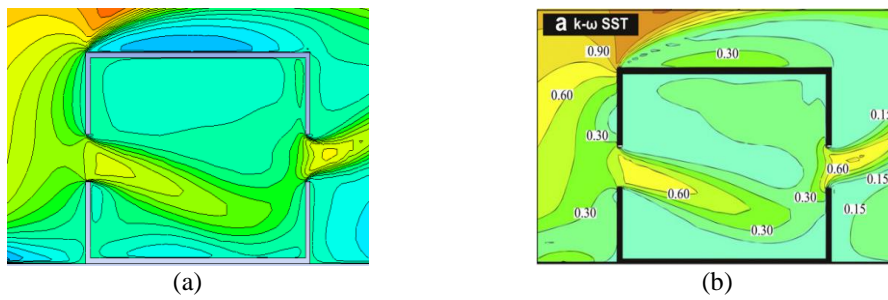
Figure 6. Validation based on velocity contour: (a) simulation result and (b) result by Ramponi and Blocken [5]
