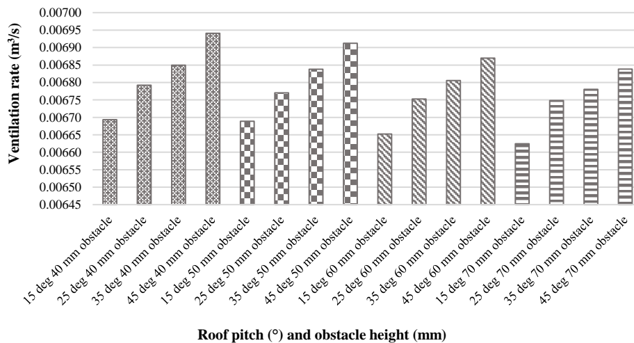
Figure 10. Ventilation rate ( \text{m}^3/\text{s} ) of gable roof with various roof pitch and obstacle height
