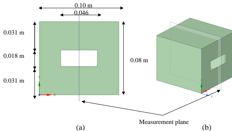
Figure 1. (a) Dimensions for the front view of the model and (b) measurement plane of reference building model [13]
