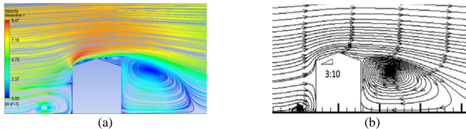
Figure 7. Validation based on the streamlines (a) simulation result of 15° roof pitch and (b) result by Tominaga et al. for roof pitch of 16.6° [8]
