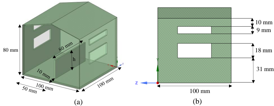
Figure 2. (a) Dimensions of the gable roof with 15^\circ roof pitch with internal obstacle and (b) front view of model dimensions
