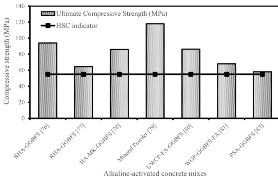
Figure 12. Alkaline-activated concrete mixes with their ultimate compressive strengths. Data adapted from Huo et al. [76], Soumya Pradhan et al. [77], Yurt and Bekar [78], Zhang et al. [79], Liang et al. [80], Marathe et al. [81], and Mengasini et al. [83]
