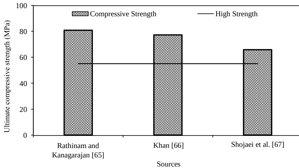
Figure 8. Ultimate compressive strength data for the different optimal alkali-activated mix. Data adapted from Rathinam and Kanadarajan [65], Khan [66] and Shojaei et al. [67]
