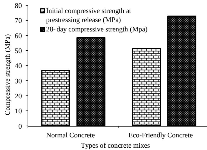
Figure 4. Types of concrete mixes and the compressive strength performance. Data adapted from Koh et al. [46]
