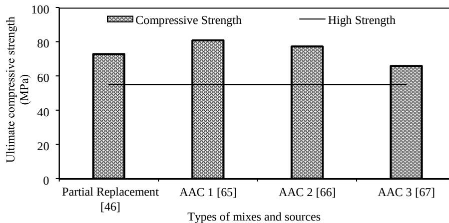
Figure 10. Ultimate compressive strength data for the different optimal alkali-activated mix. Data adapted from Koh et al. [46], Rathinam and Kanadarajan [65], Khan [66] and Shojaei et al. [67]
