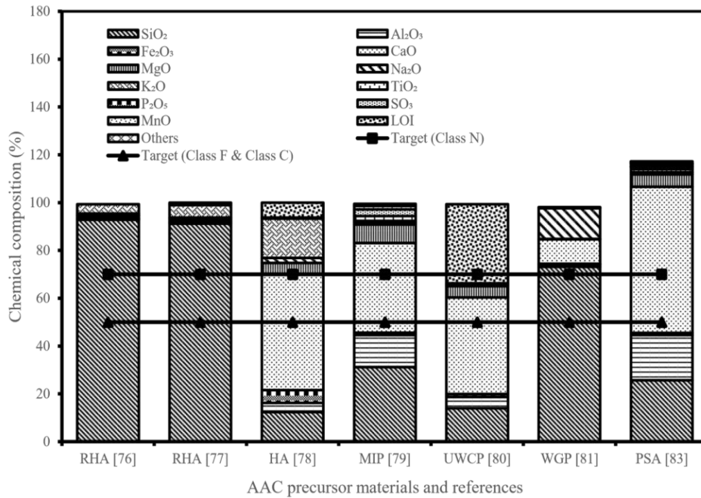
Figure 13. Chemical composition of precursor materials. Data adapted from Huo et al. [76], Soumya Pradhan et al. [77], Yurt and Bekar [78], Zhang et al. [79], Liang et al. [80], Marathe et al. [81], and Mengasini et al. [83]
