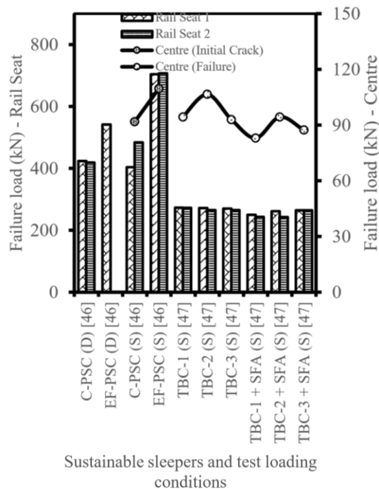
Figure 5. Types of concrete railway sleepers mixes and bending strength of PSC sleepers. Data adapted from Koh et al. [46] and Prabhu et al. [47]
