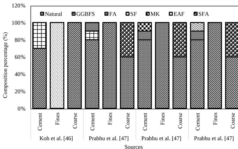
Figure 3. Concrete railway sleeper mixes. Data adapted from Koh et al. [46] and Prabhu et al. [47]
