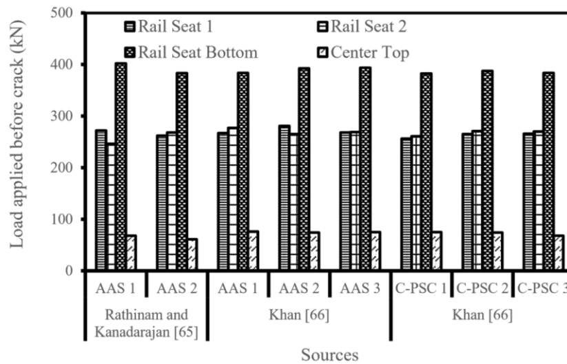
Figure 9 Performance of different alkali-activated concrete railway sleepers. Data adapted from Rathinam and Kanadarajan [65] and Khan [66]
