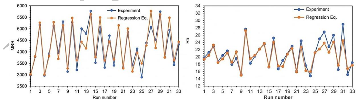
Figure 5. Comparison of MRR and R_a between findings from experiments and the regression model for different run numbers
