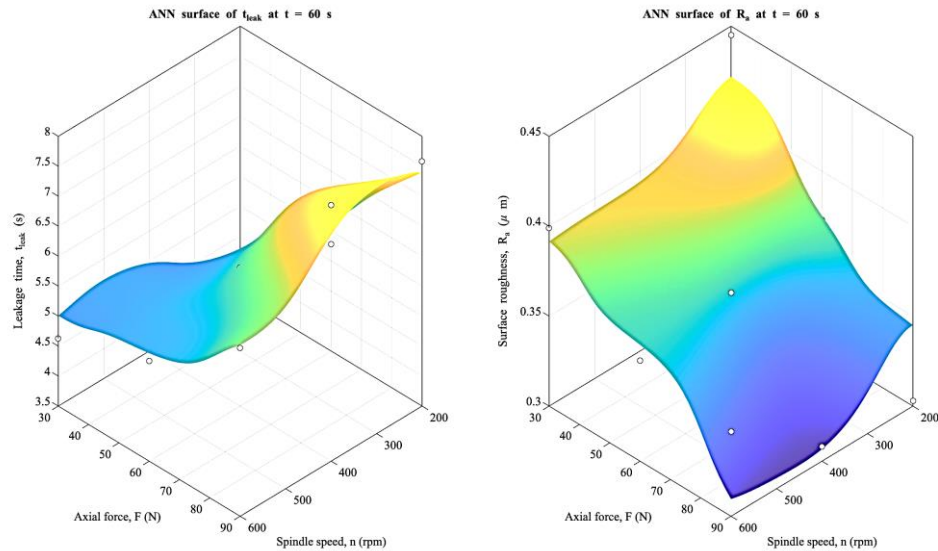
Figure 11. Response surfaces obtained from the ANN surrogate model for (a) leakage time t_{\text{leak}} and (b) surface roughness R_a as functions of spindle speed n and axial force F at a fixed lapping time of t = 60 s. Symbols indicate the experimental design points
