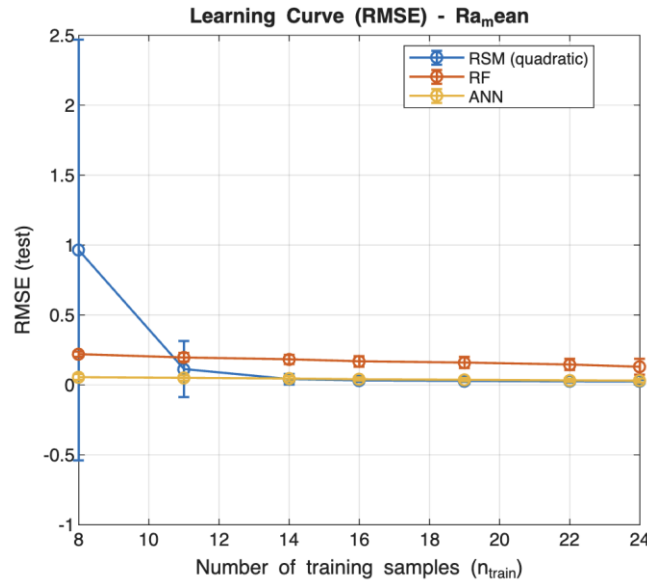
Figure 6. Learning curve of test RMSE versus number of training samples ( n_{train} ) for surface roughness ( Ra_{mean} ), comparing quadratic RSM, random forest, and artificial neural network. Error bars denote \pm 1 standard deviation across the repeated resampling runs
