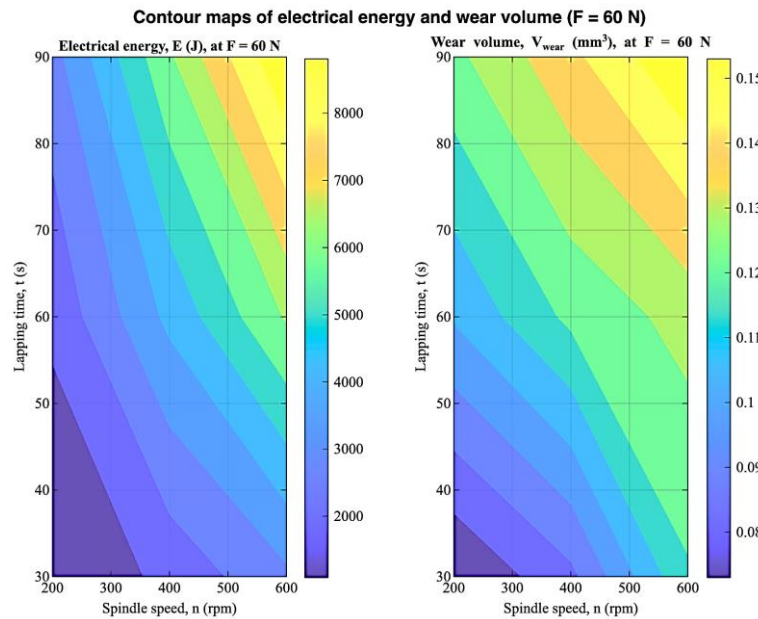
Figure 5. Contour maps of (a) electrical energy E and (b) wear volume V_{\text{wear}} as functions of spindle speed n and lapping time t at a constant axial force of F = 60\text{ N}
