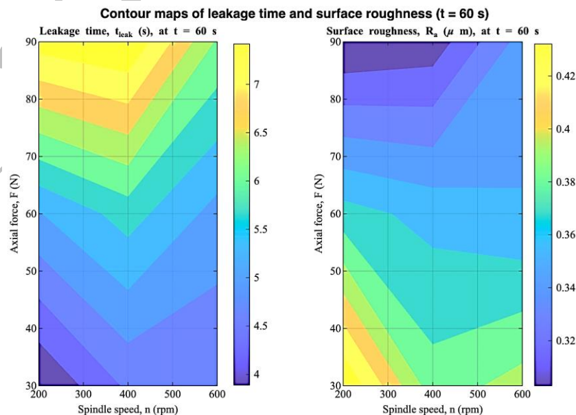
Figure 4. Contour maps of (a) leakage time t_{\text{leak}} and (b) surface roughness R_a as functions of spindle speed n and axial force F at a lapping time of t = 60\text{s}
