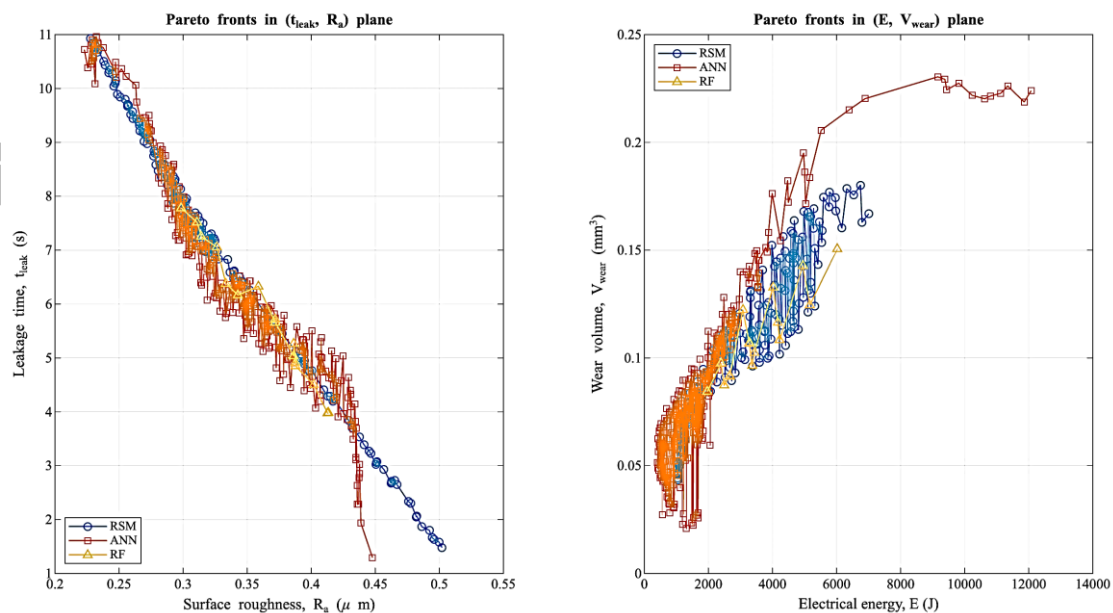
Figure 12. Pareto fronts obtained with NSGA-II using RSM, ANN and RF surrogates in (a) the (t_{\text{leak}}, R_a) plane and (b) the (E, V_{\text{wear}}) plane
