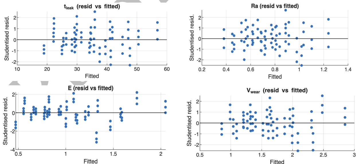
Figure 9. Studentised residuals versus fitted values for the quadratic RSM model using the 81 raw measurements (3 replicates \times 27 design points) for t_{leak} , Ra , E , and V_{wear}
