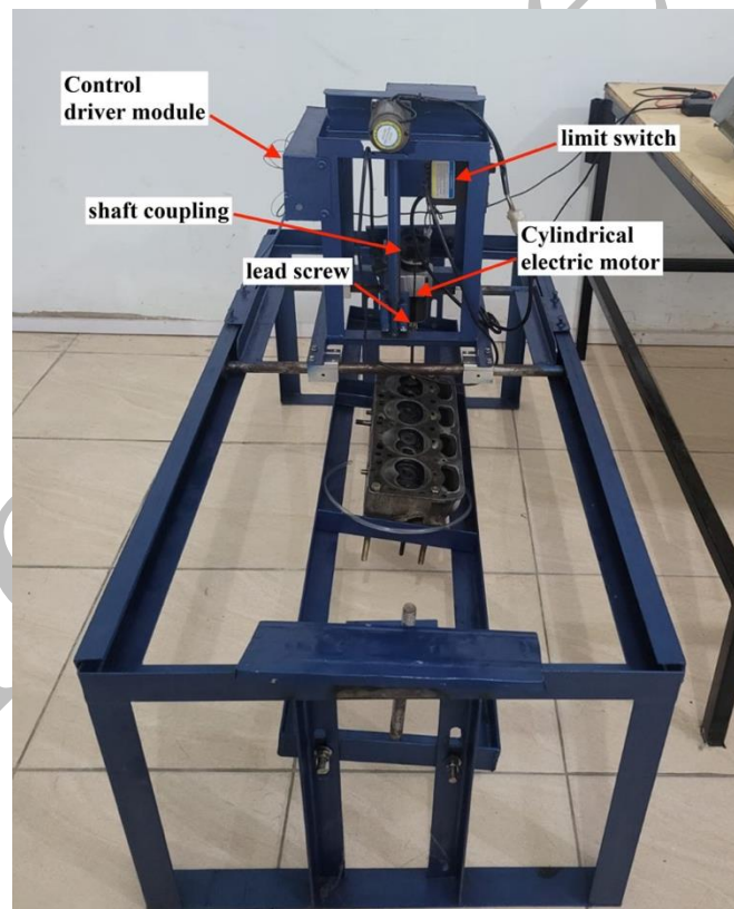
Figure 1. automatic valve lapping machine and cylinder head fixture
