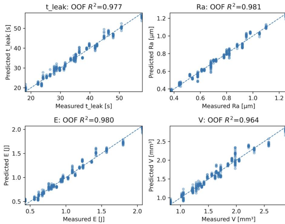
Figure 8. Out-of-fold parity plots for quadratic RSM (repeated 5-fold CV, 20 repeats)
