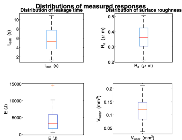
Figure 2. Box and whisker plots of the measured responses: (a) leakage time t_{\text{leak}} , (b) surface roughness R_a ,
