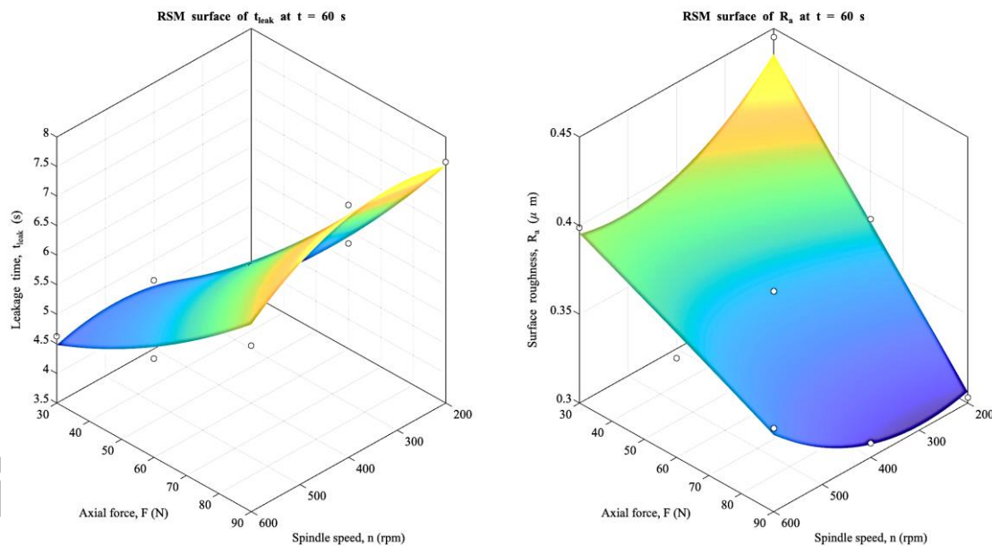
Figure 10. Response surfaces obtained from the quadratic RSM for (a) leakage time t_{leak} and (b) surface roughness R_a as functions of spindle speed and axial force at a fixed lapping time of t = 60 s. Symbols indicate the experimental design points
