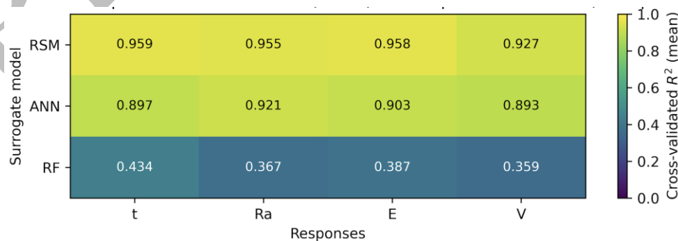
Figure 7. Heatmap of cross-validated R^2 (mean) from repeated 5-fold CV (20 repeats)
