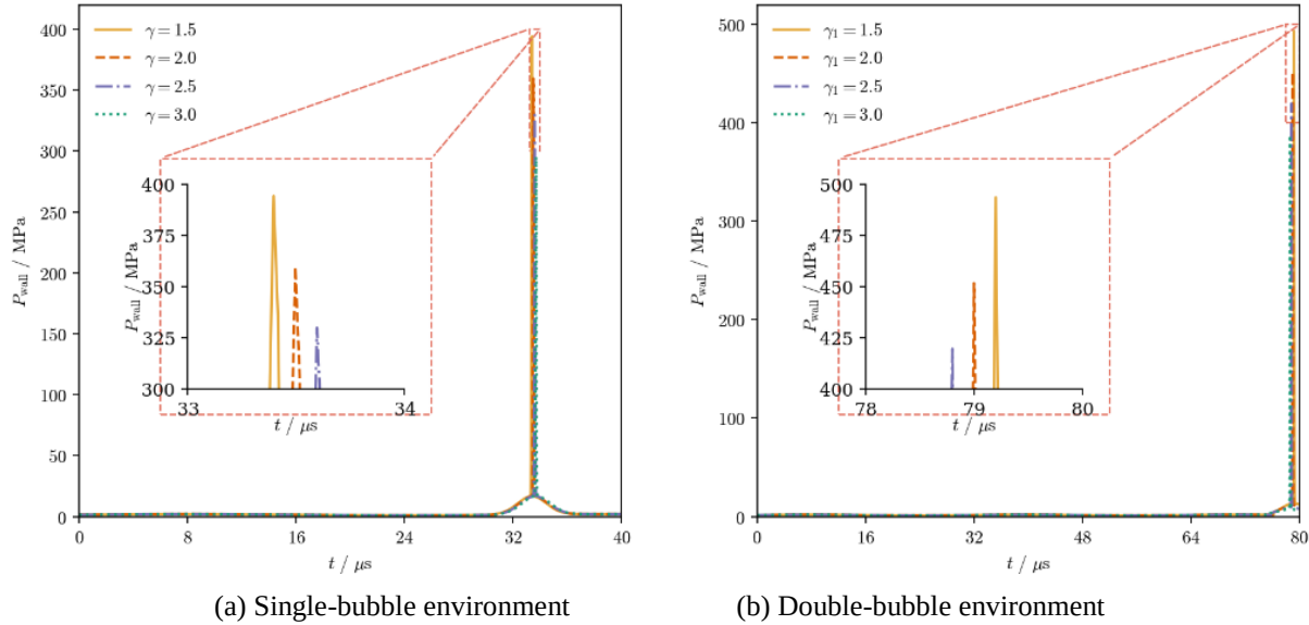
Figure 16. Wall impact pressure at different dimensionless distances
