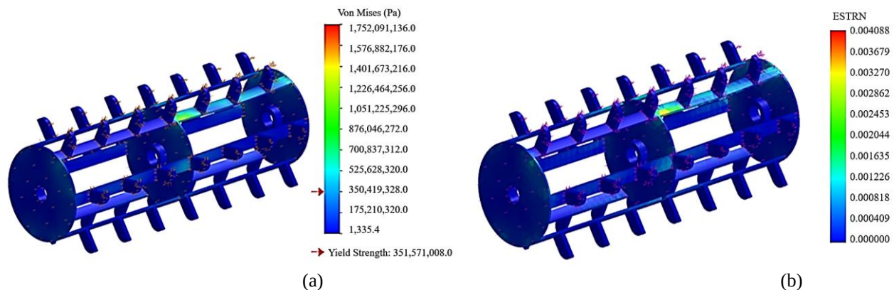
Figure 3. Static stress (a) and strain (b) simulation results of the peg-tooth cylinder
