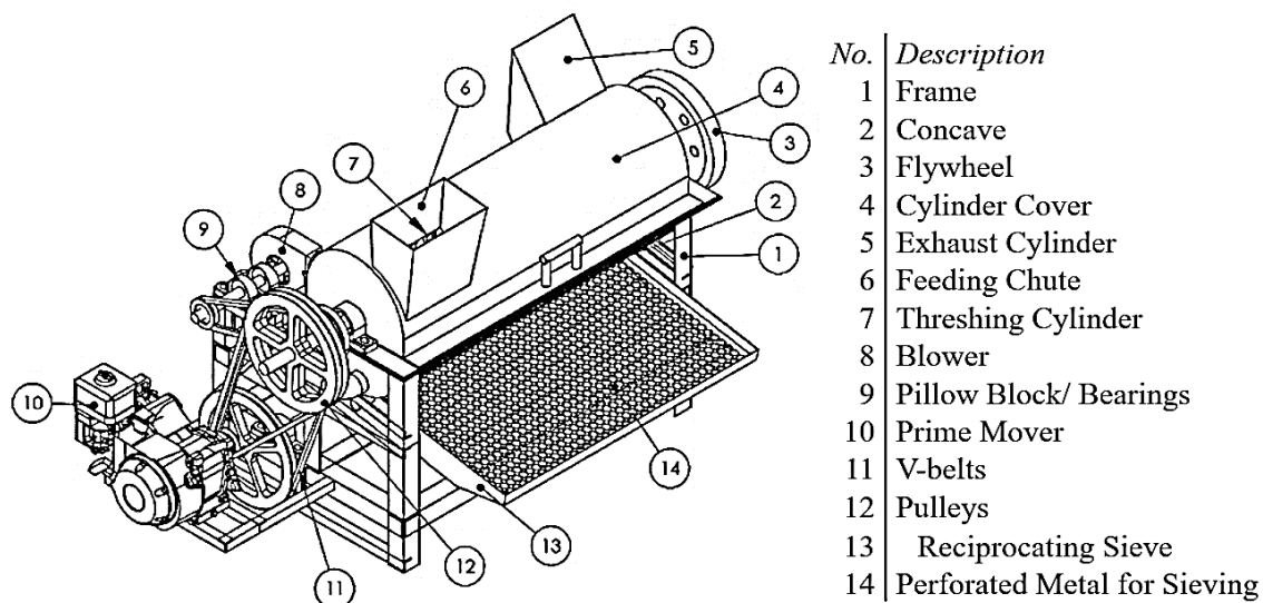
Figure 2. Two-dimensional wireframe drawing of the Adlai threshing machine
