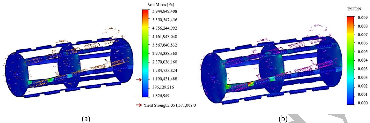
Figure 4. Static stress (a) and strain (b) simulation results of the rasp bar cylinder
