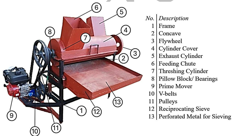
Figure 5. Fabricated Adlai threshing machine
