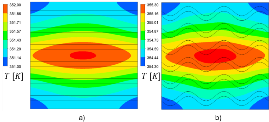
Figure 6. 1Baseplate temperature distribution of a) HS1 and b) HS2 from CFD simulation results
