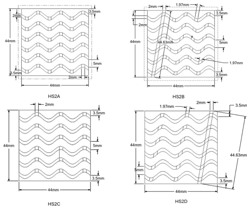
Figure 12. 2Four additional wavy heat sinks were created by cutting the continuous fins into discrete sections
