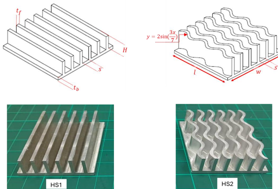
Figure 1. Parameters of the CNC-machined heat sink
