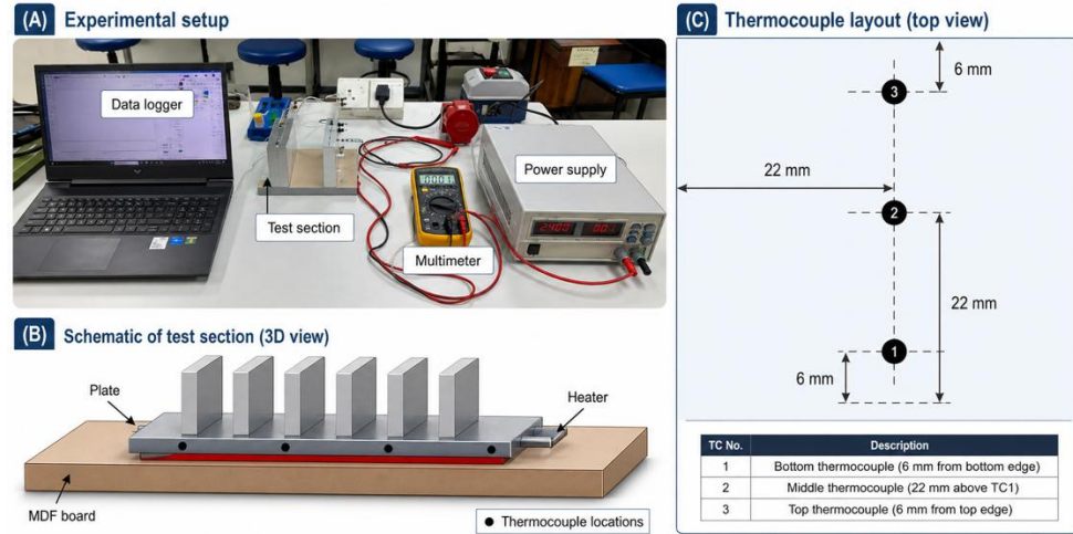
Figure 2. (A) Illustration of the experiment setup to measure heat sink thermal performance; (B) Schematic of the test section, and (C) locations of the thermocouples under the heat sink
