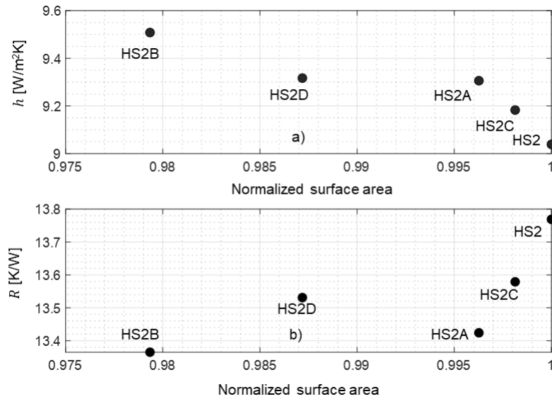
Figure 14. Relationship between thermal resistance, heat transfer coefficient and surface area of the heat sinks
