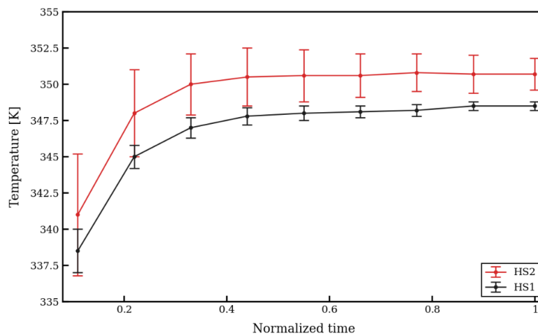
Figure 5. Temperature measurements at the base of HS1 and HS2
