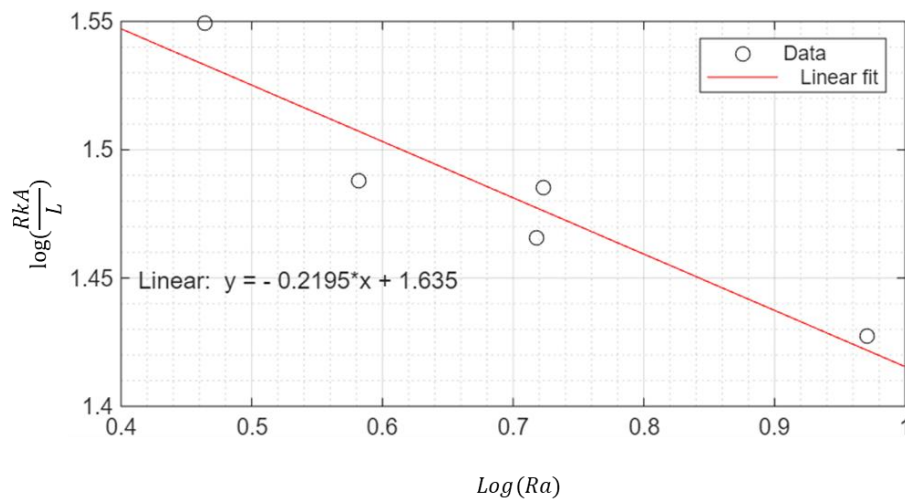
Figure 15. Relationship between thermal resistance and Rayleigh number
