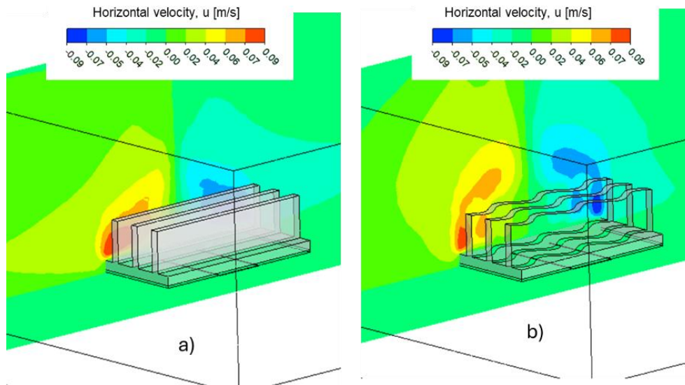
Figure 8. Horizontal velocity contour at midplane inside fin channel of a) HS1 and b) HS2
