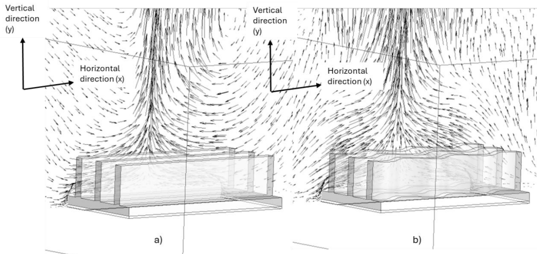
Figure 9. Velocity vector plotted at midplane inside fin channel of a) HS1 and b) HS2
