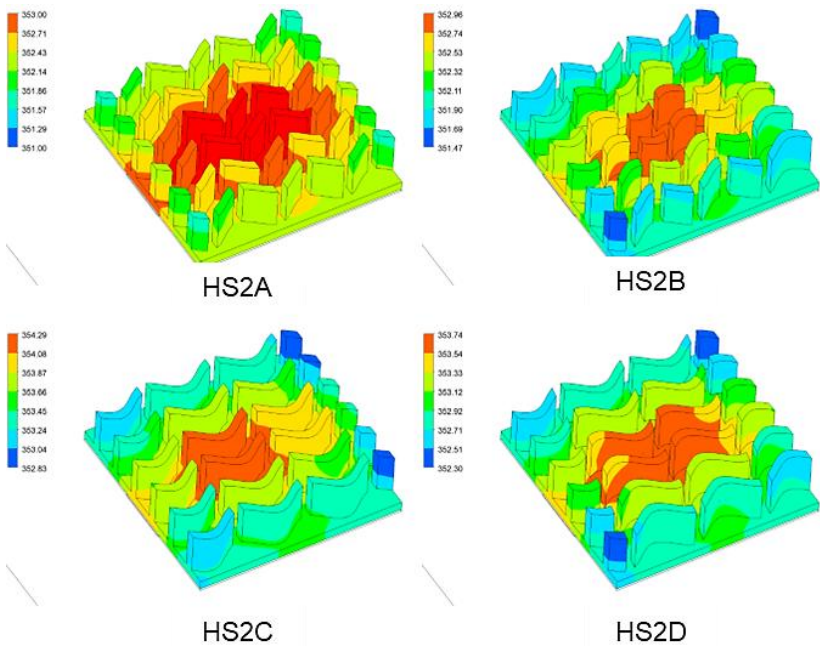
Figure 13. Surface temperature contour of the crosscut heat sinks
