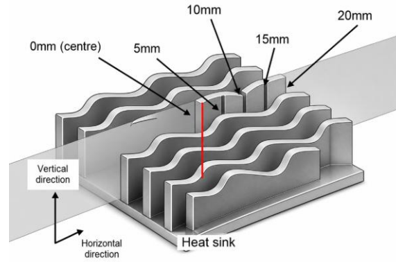
Figure 10. Location of midplane and lines for extracting horizontal velocity profiles inside the fin channel
