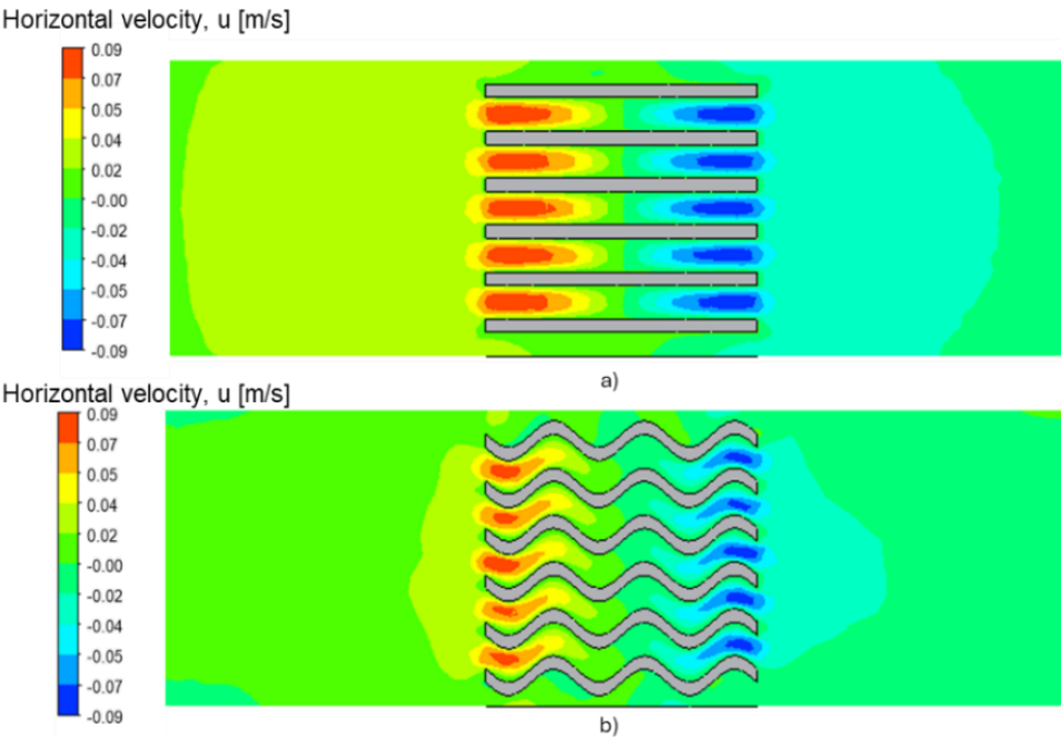
Figure 7. Top view of horizontal velocity contour at fin mid-height of a) HS1and b) HS2
