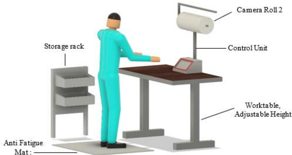
Figure 3. Redesign workstation layout with ergonomic enhancements.
