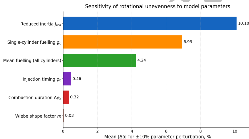
Figure 11. Sensitivity of the rotational-unevenness coefficient to a \pm 10\% change in each model parameter
