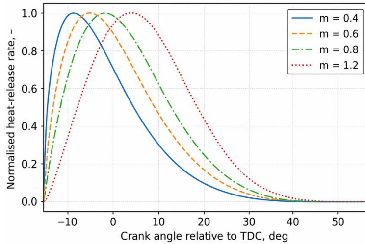
Figure 3. Heat-release rate for several values of the Wiebe shape factor m
