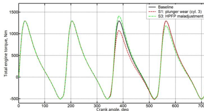
Figure 5. Engine torque for the baseline and two fault scenarios
