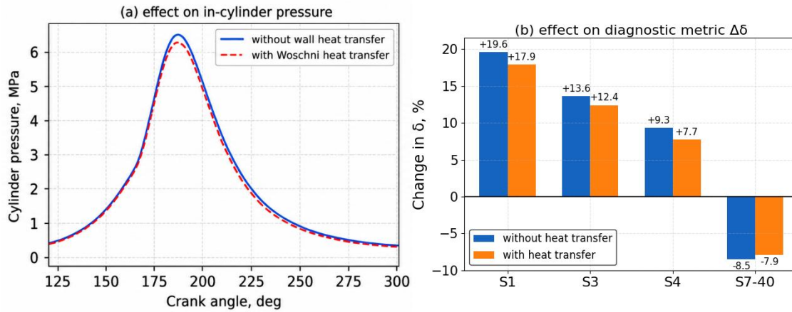
Figure 9. Robustness to wall heat transfer: effect on cylinder pressure (left) and on the diagnostic metric \Delta\delta (right)
