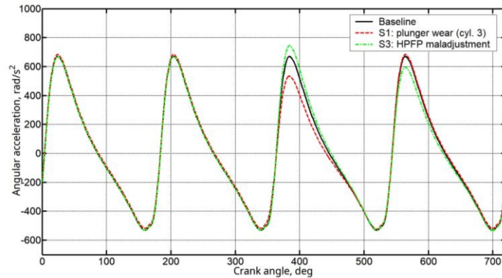
Figure 6. Crankshaft angular acceleration for the baseline and two fault scenarios
