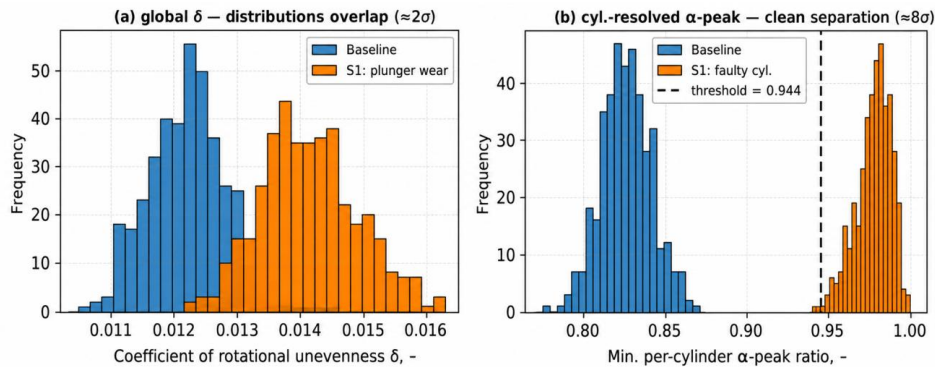
Figure 12. Monte-Carlo separation of healthy and faulty engine by the global coefficient (left) and by the cylinder-resolved peak-acceleration ratio (right)
