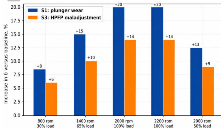
Figure 10. Increase in rotational unevenness for fault S1 across speed and load
