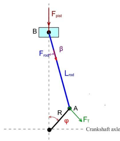
Figure 2. Forces and geometry of the crank mechanism
