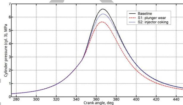
Figure 4. In-cylinder pressure for the baseline and two fault scenarios
