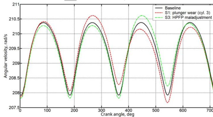
Figure 7. Fluctuation of crankshaft angular velocity
