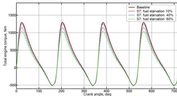
Figure 8. Effect of fuel-filter restriction on engine torque
