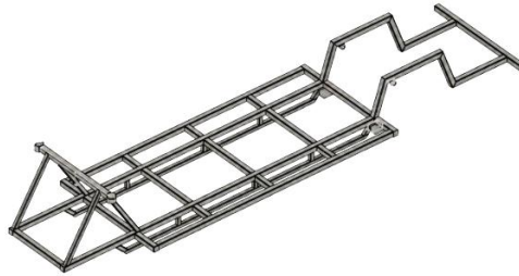
Figure 3. Ladder-frame chassis model used for finite element analysis
