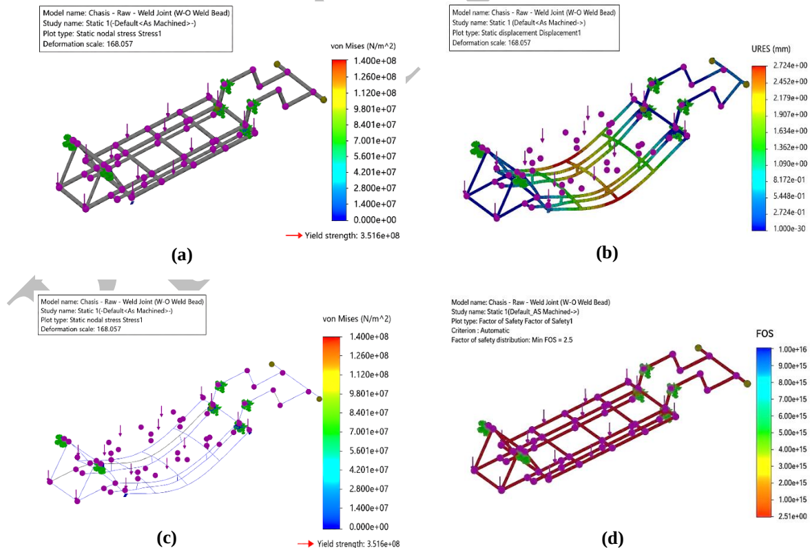
Figure 4. Finite-element model and structural response: (a) static nodal stress plot with applied boundary conditions and loading, (b) resultant displacement, (c) von Mises stress, and (d) factor of safety
