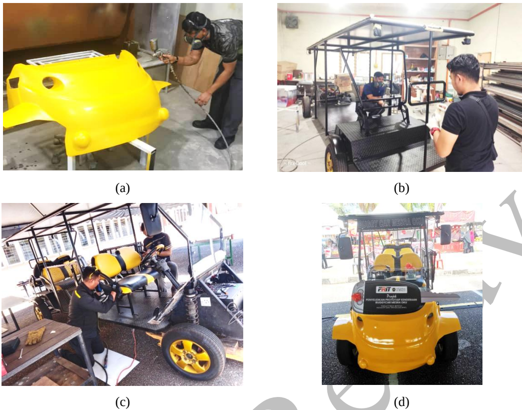
Figure 6. Prototype fabrication and deployment stages: (a) body-panel finishing, (b) frame assembly, (c) on-site commissioning, and (d) rear view during demonstration
