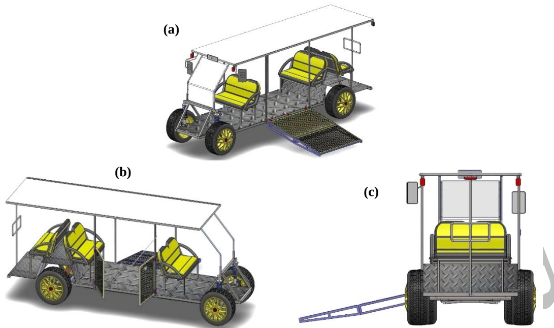
Figure 2. CAD configurations of the wheelchair-accessible campus buggy: (a) overall concept, (b) side-access and seating arrangement, and (c) rear ramp-deployment geometry
