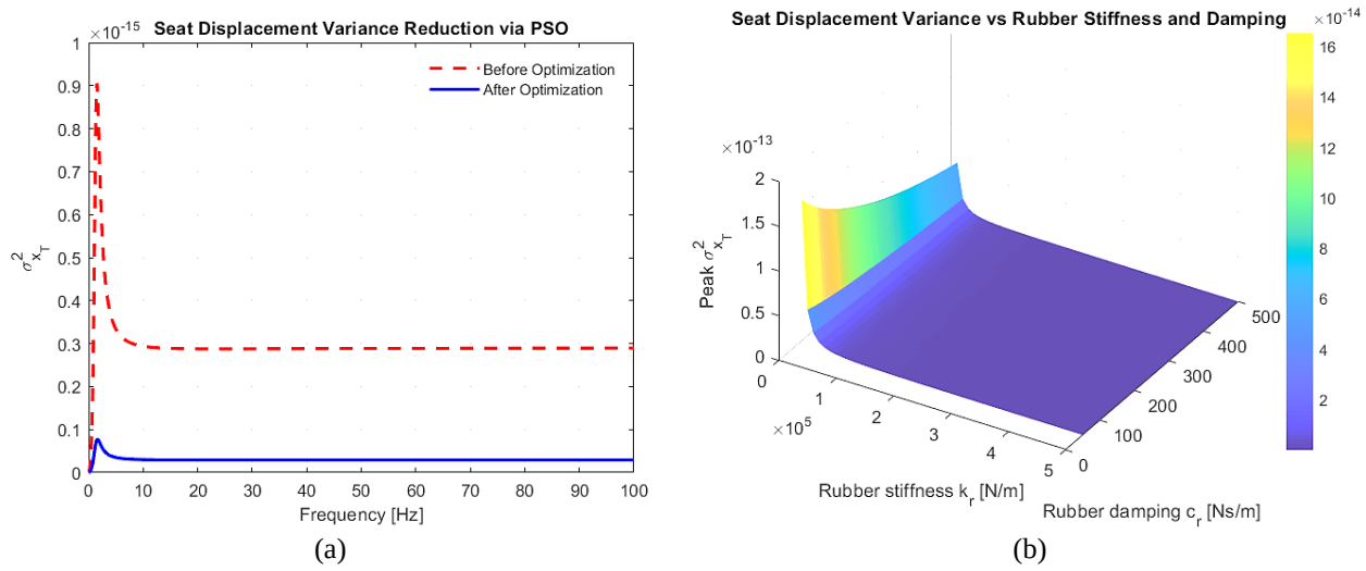
Figure 9. Seat displacement (a) variance ( \sigma_{x_t}^2 ) vs (b) frequency
