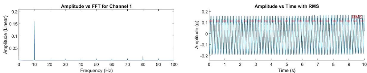
Figure 6. Example FFT and time waveform of each damper (at 10 Hz sinusoidal excitation)
