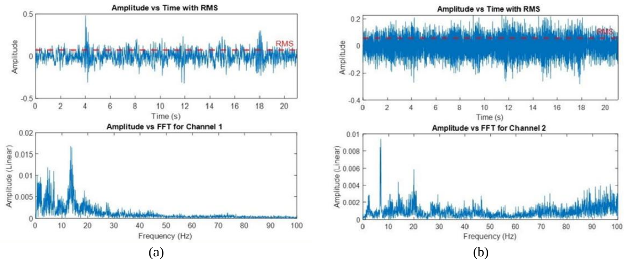
Figure 5. Vibration data from (a) bus seat floor, (b) vibration data from seat cushion (right) at 60 km/h
