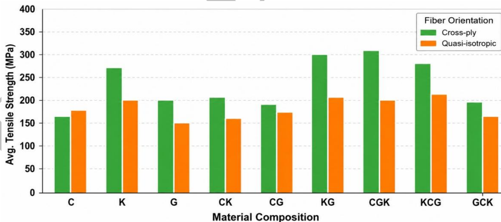
Figure 4. Fiber orientation effects on average tensile strength
