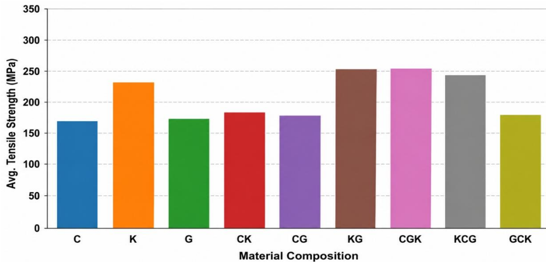
Figure 3. Material compositional effects on average tensile strength
