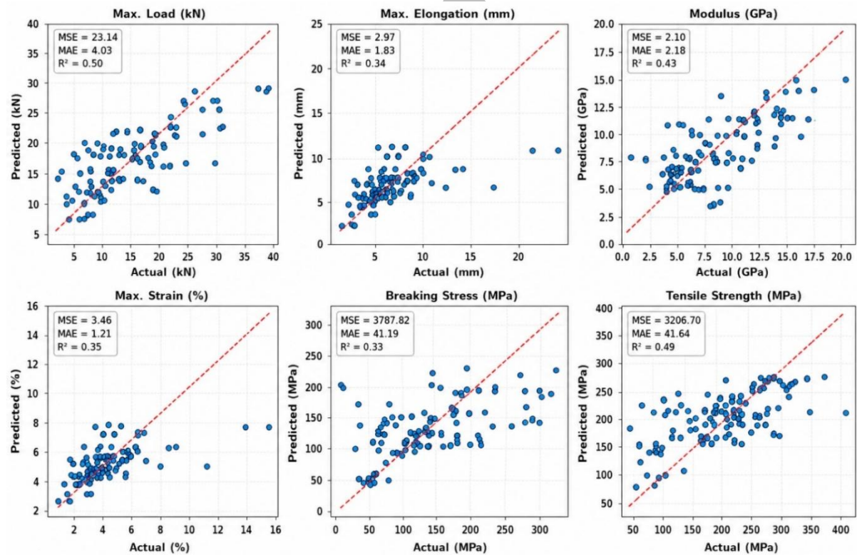
Figure 16. Actual versus predicted plot of SGB for tensile properties as target features
