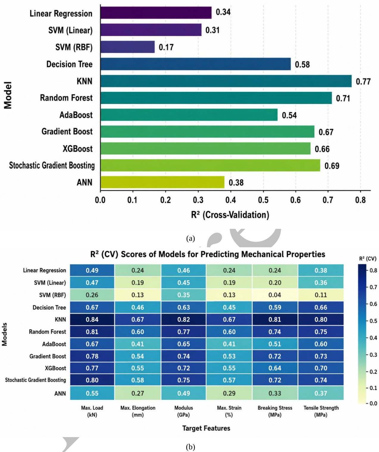
Figure 12. K-fold cross-validation: (a) R^2 per model and (b) Heat map of R^2 per target for tensile properties as target features
