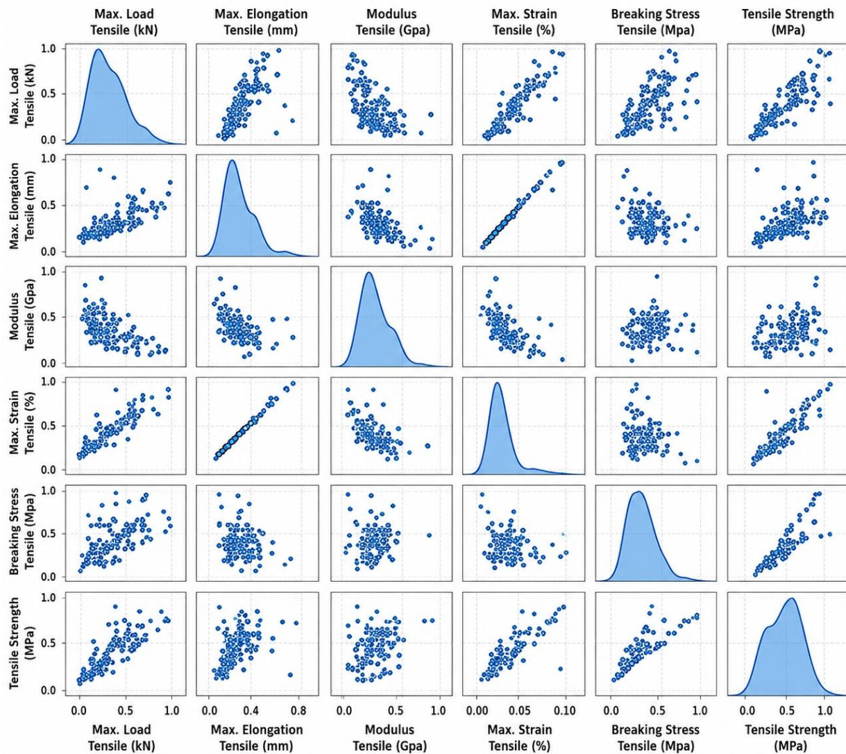
Figure 8. Pair plots of scaled tensile properties as target features
