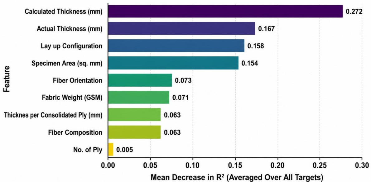
Figure 10. Feature importance of tensile properties as target features
