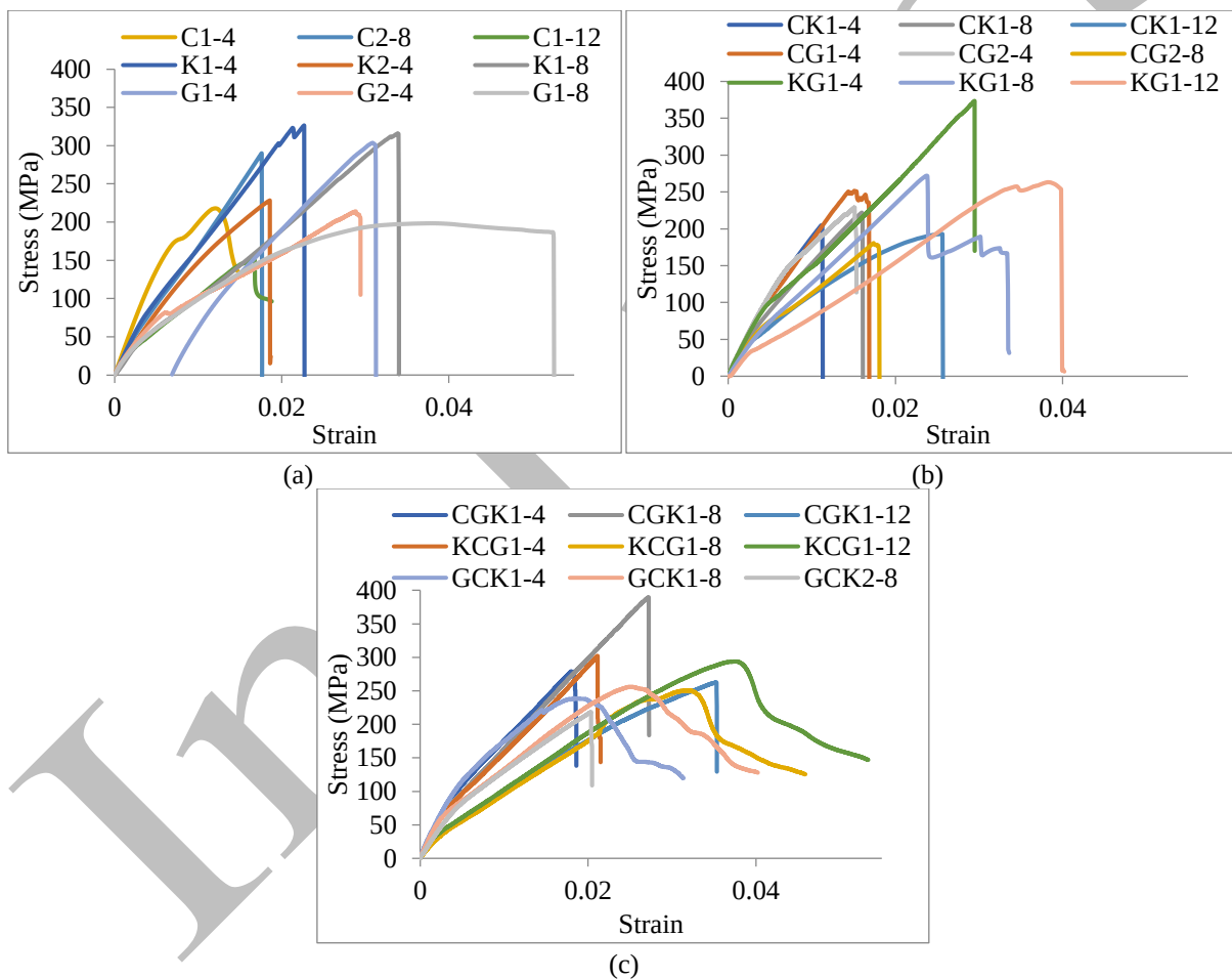
Figure 2. Stress versus Strain curves: (a) for 100%; (b) for 50% + 50%; and (c) for 50% + 25% + 25% compositions
