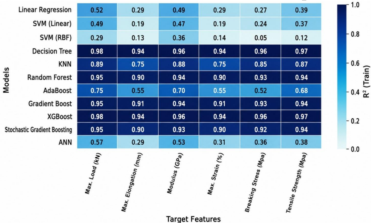
Figure 11. Heat map of models' training R 2 per target for tensile properties as target features
