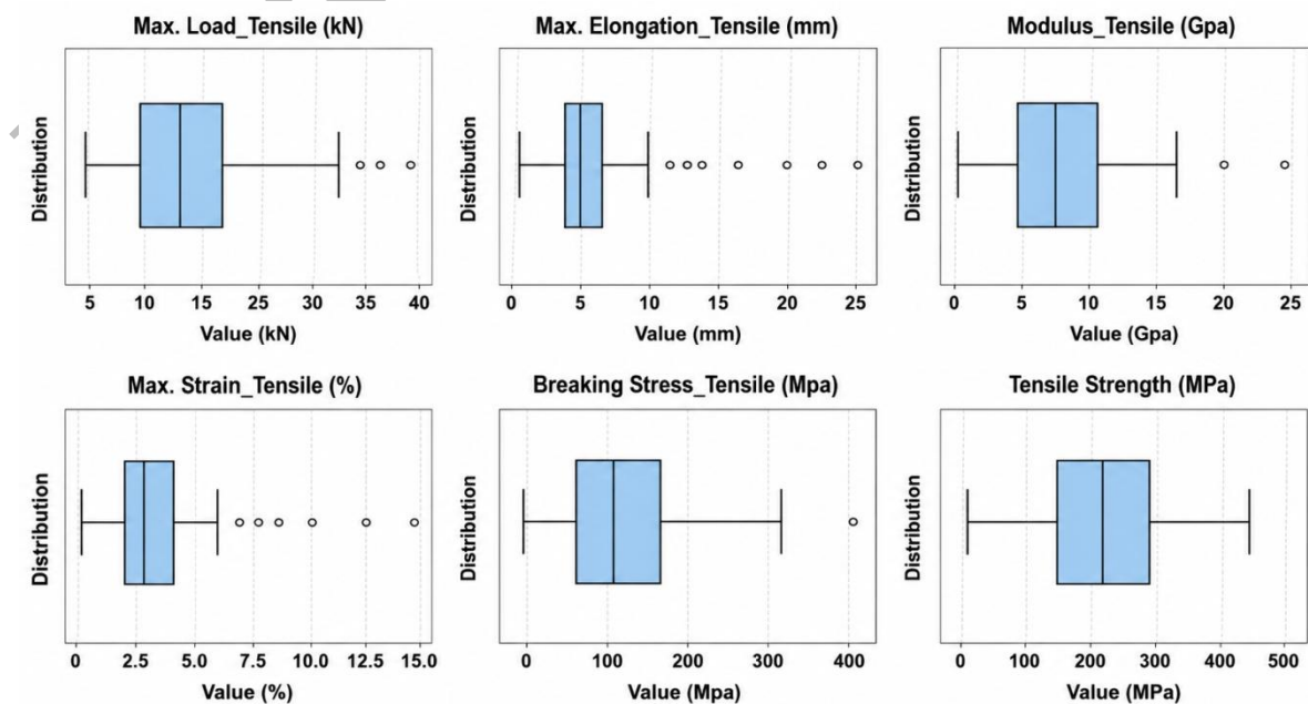
Figure 7. Boxplot of outliers of tensile properties as target features
