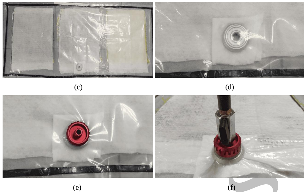
Figure 1. Manual wet lap of vacuum bagging technique: (a) Bleeder fabric double layering; (b) Vacuum connector (1 st part) setting; (c) Polythene sheet (top) layering and sealant tape closing; (d) Hole making above 1st part of vacuum connector for air exhaustion; (e) Vacuum connector (2 nd part) setting; (f) Vacuum connector (2 nd part) and air exhaust pipe connecting
