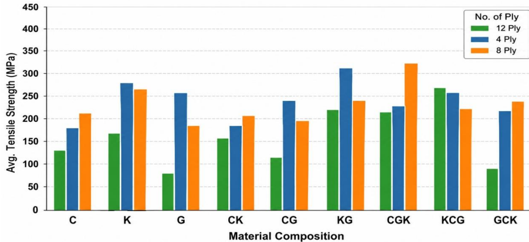
Figure 5. The effect of the number of plies on the average tensile strength
