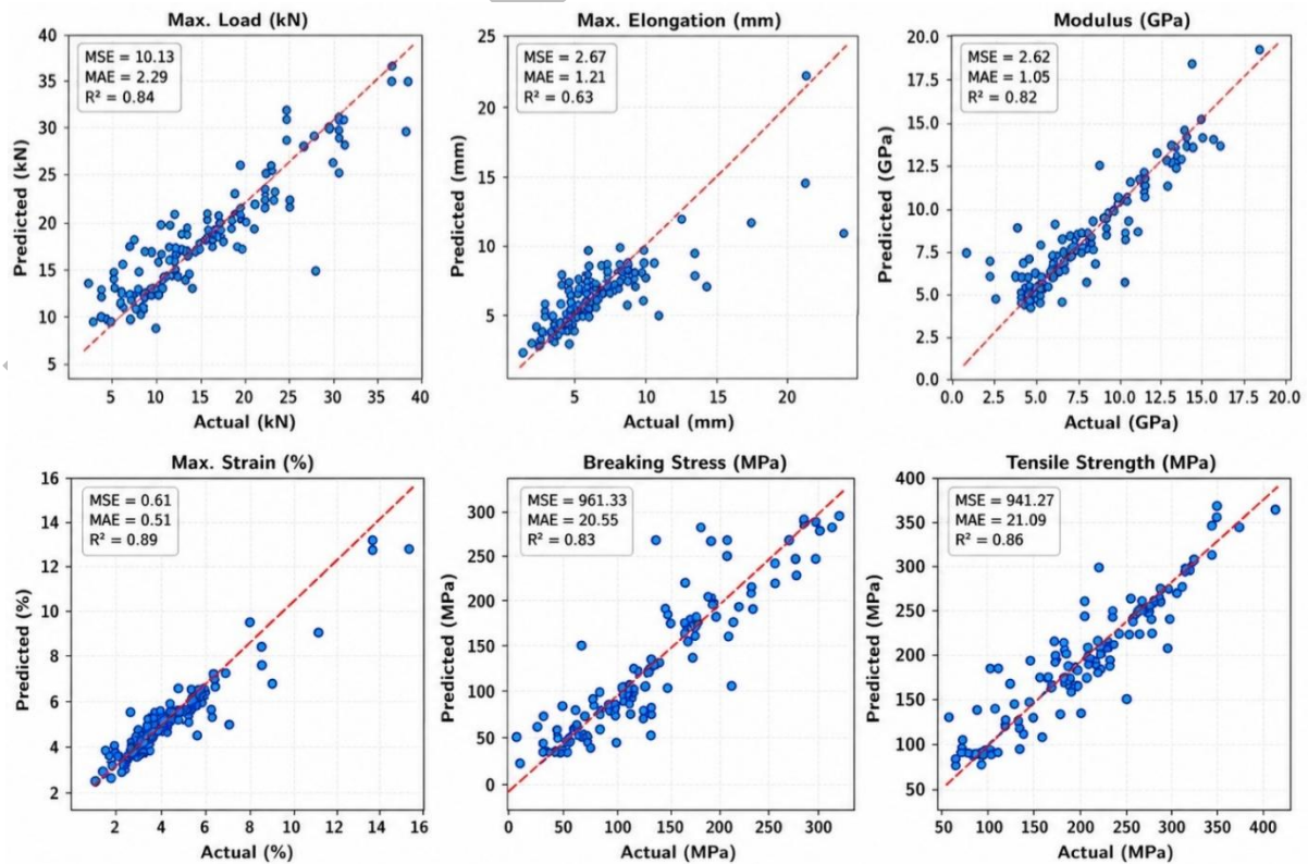
Figure 15. Actual versus predicted plot of KNN for tensile properties as target features
