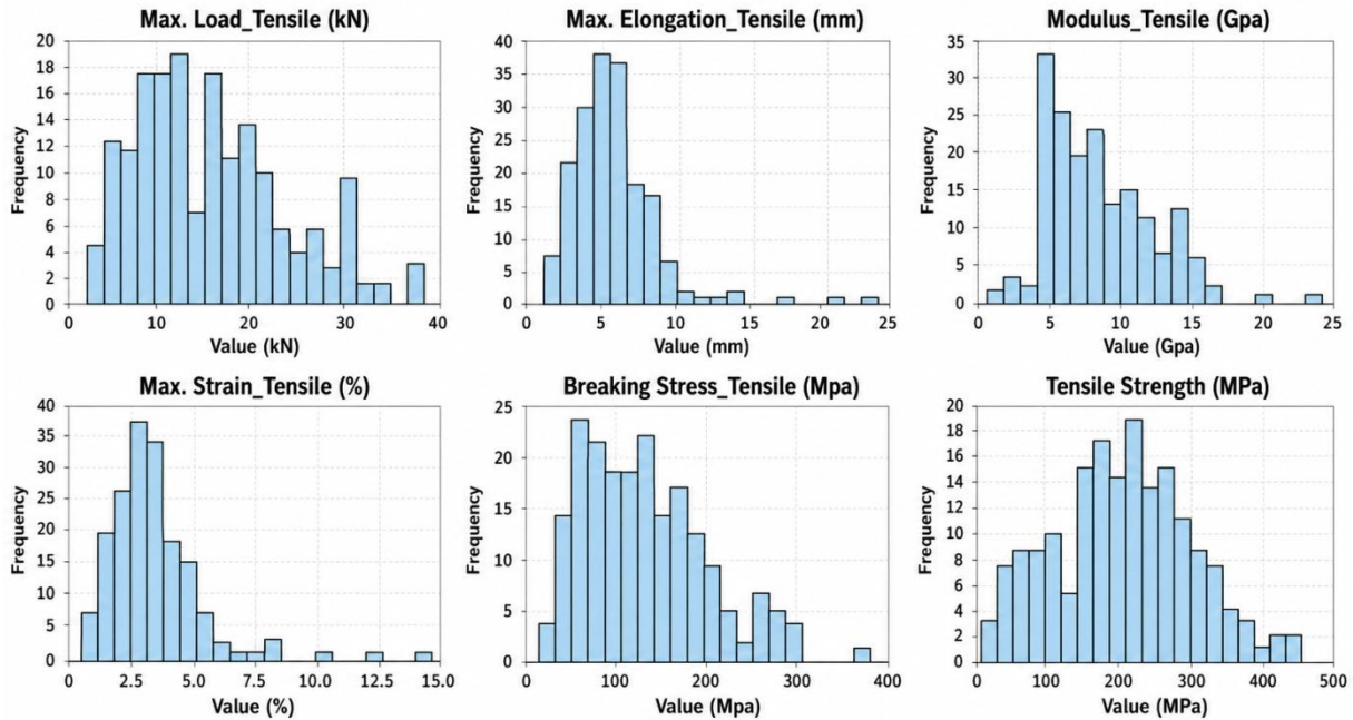
Figure 6. Data distribution of tensile properties as target features
