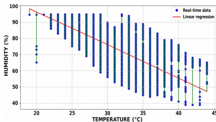
Figure 5. Correlation between air temperature and relative humidity during fan-assisted cooling ( r = -0.7287 )
