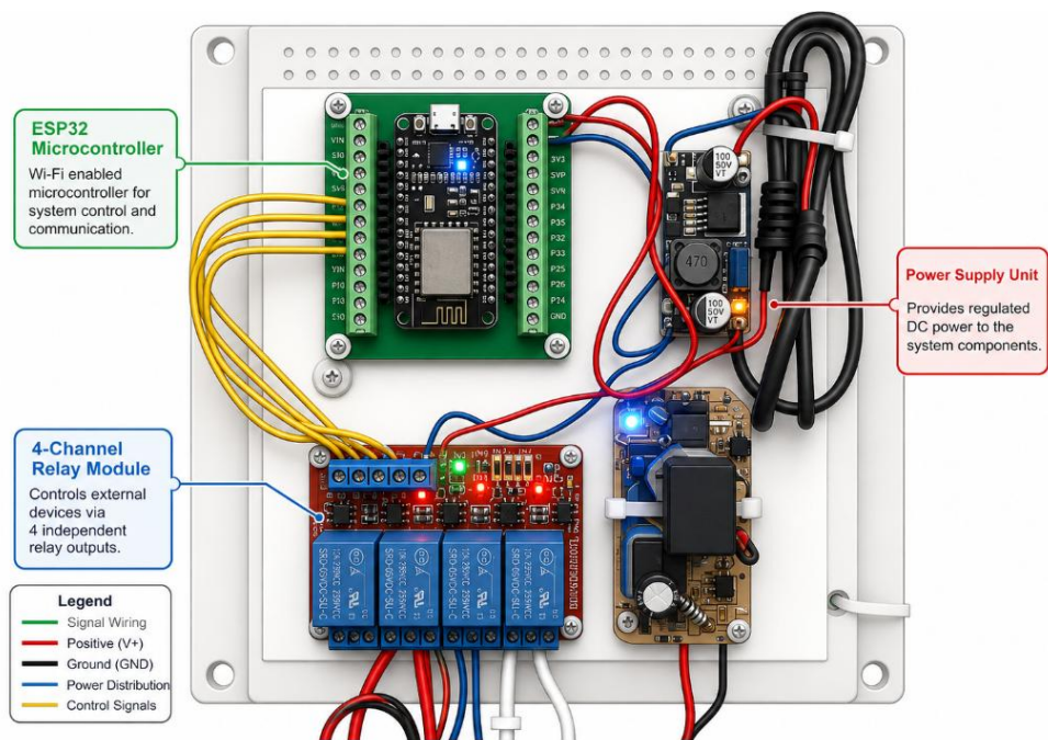
Figure 14. Electrical control system for fan and cooling relays
