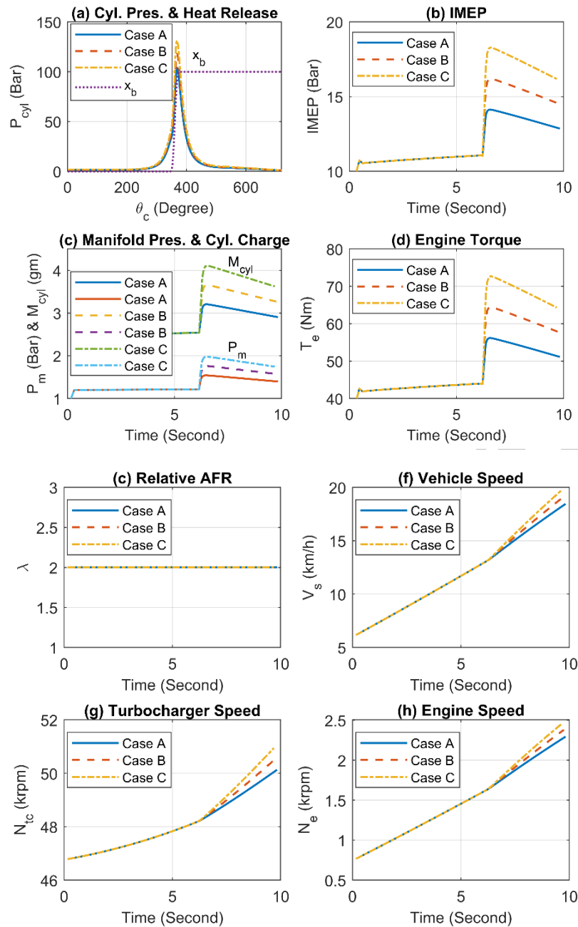
Figure 2. Effect of boosting assistance pressure on vehicle acceleration using the test's initial values: N_e = 750 \text{ rpm} , \lambda = 2.0 , and 1 st Gear Ratio. Case A: Boosting assistance P_a = 1.75 \text{ bar} ; Case B: Boosting assistance P_a = 2.0 \text{ bar} ; Case C: Boosting assistance P_a = 2.25 \text{ bar}
