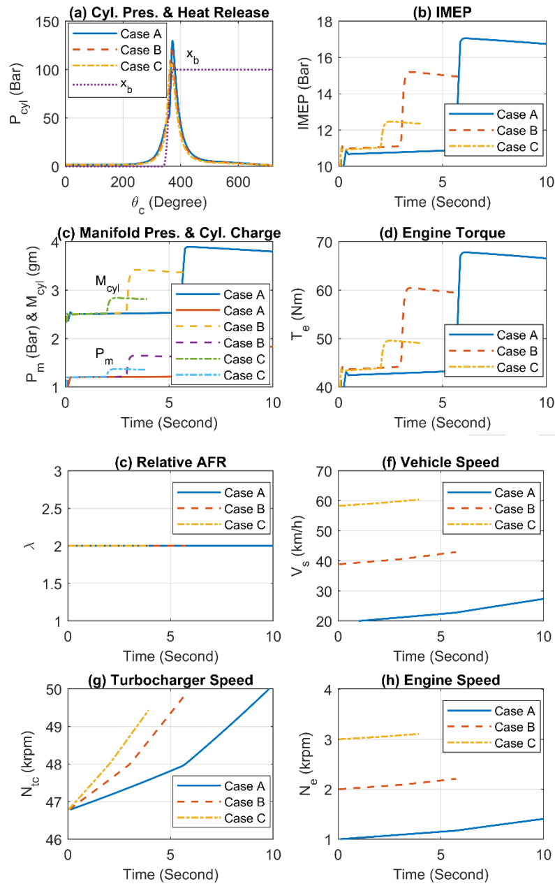
Figure 5. Effect of road load dynamics on vehicle acceleration using the test's initial values: P_a = 2.0 \text{ bar} , \lambda = 2.0 , and 3 rd Gear Ratio. Case A: Boosting assistance at N_e = 1000 \text{ rpm} ; Case B: Boosting assistance at N_e = 2000 \text{ rpm} ; Case C: Boosting assistance at N_e = 3000 \text{ rpm}
