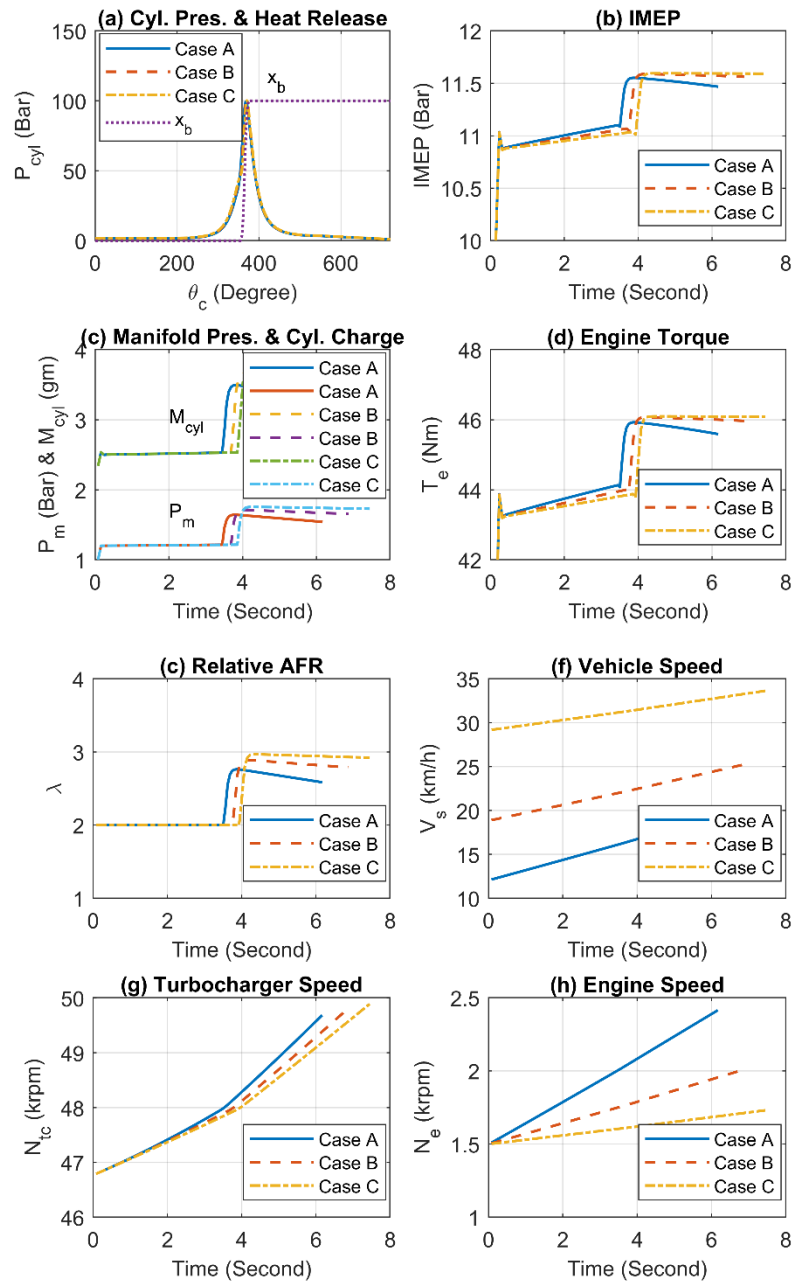
Figure 6. Effect of combined factors on vehicle acceleration using the test's initial values: P_a = 2.0 \text{ bar} , \lambda = 2.0 , and N_e = 1500 \text{ rpm} . Case A: Boosting assistance at 1 st Gear Ratio; Case B: Boosting assistance at 2 nd Gear Ratio; Case C: Boosting assistance at 3 rd Gear Ratio
