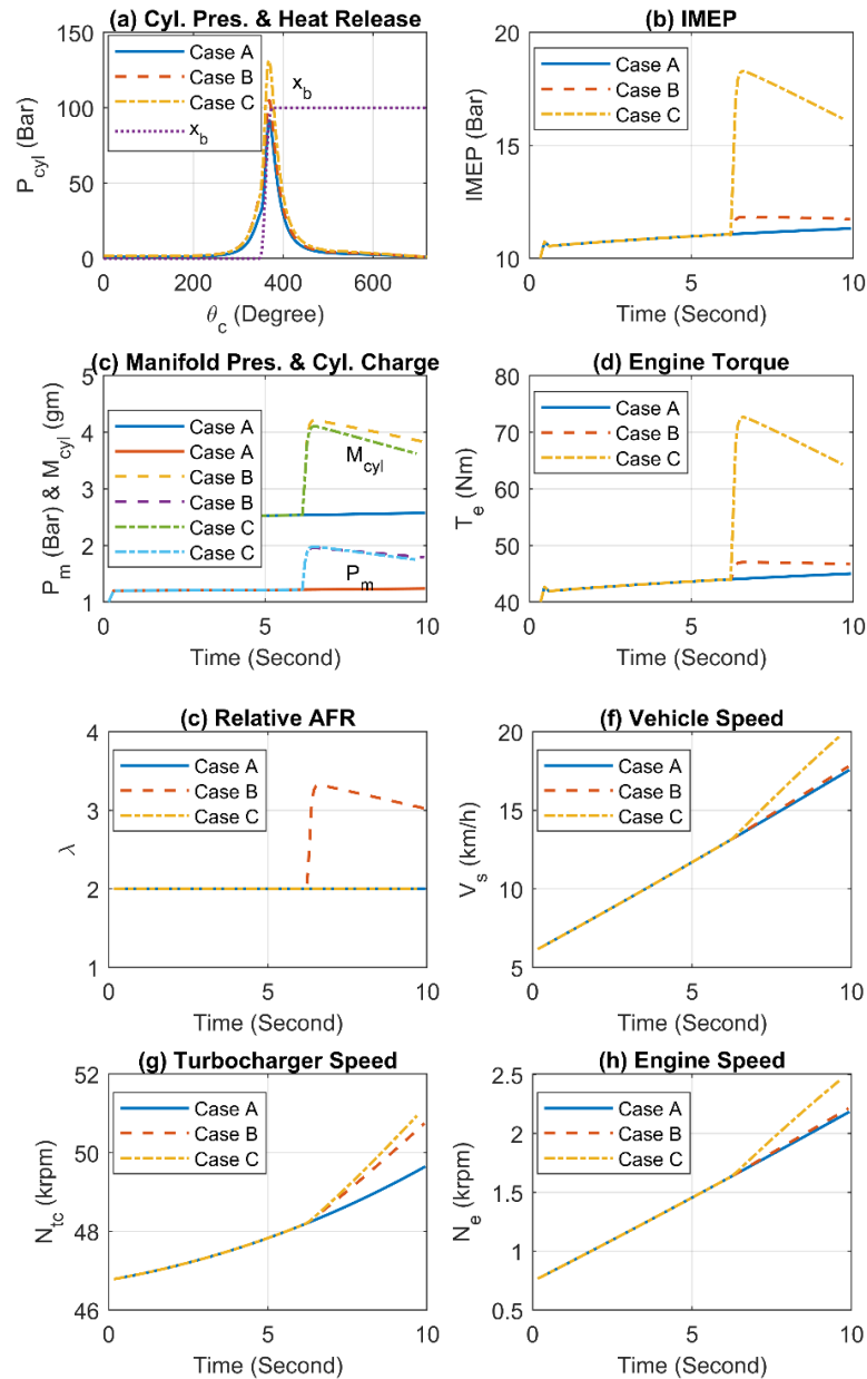
Figure 3. Effect of air-fuel ratio on vehicle acceleration using initial values: N_e = 750 \text{ rpm} , \lambda = 2.0 , P_a = 2.25 \text{ bar} and 1 st Gear Ratio. Case A: Without boosting assistance and constant AFR; Case B: With boosting assistance and constant AFR; Case C: With boosting assistance and variable AFR
