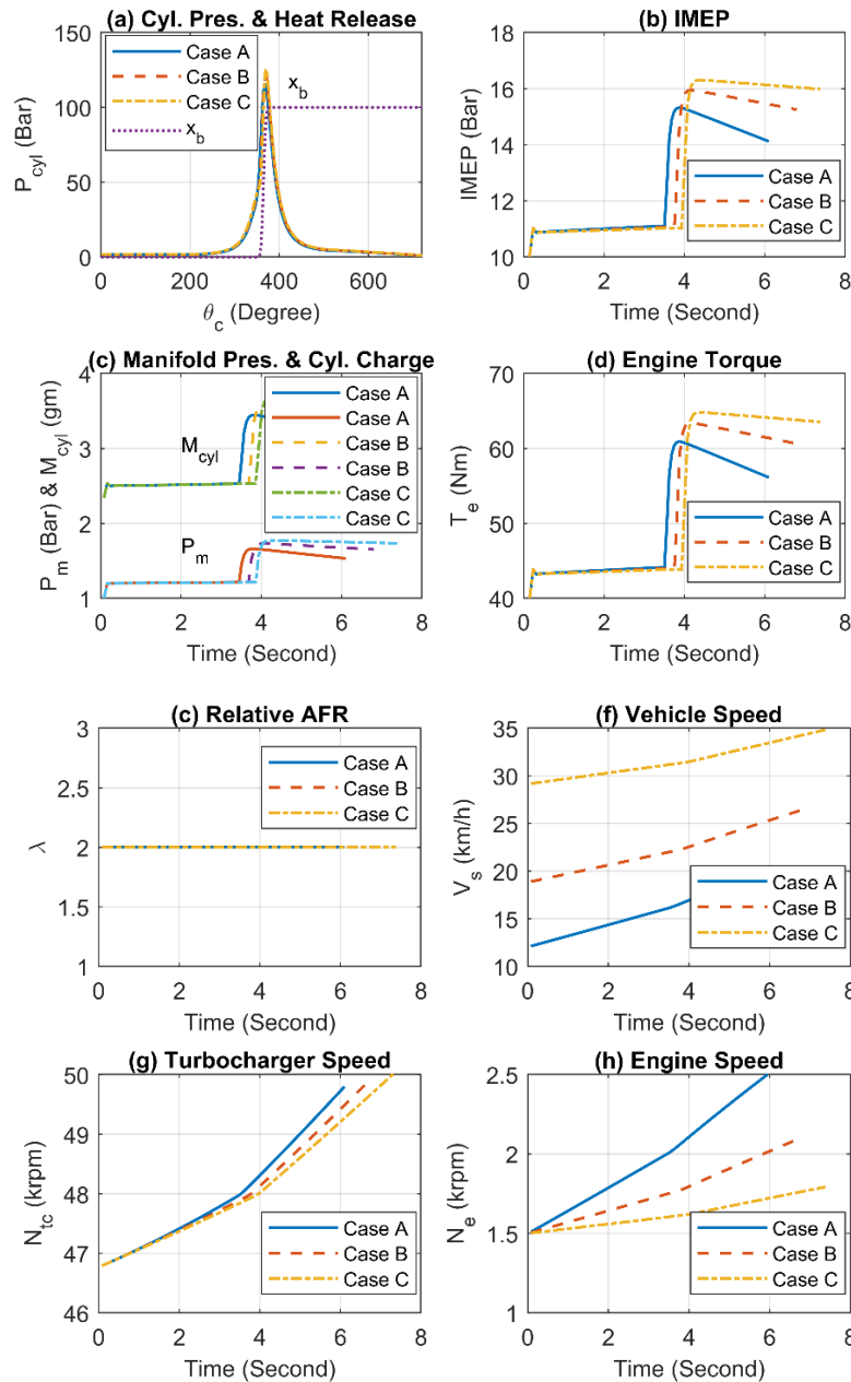
Figure 4. Effect of powertrain dynamics on vehicle acceleration using the test's initial values: P_a = 2.0 \text{ bar} , \lambda = 2.0 , and N_e = 1500 \text{ rpm} . Case A: Boosting assistance at 1 st Gear Ratio; Case B: Boosting assistance at 2 nd Gear Ratio; Case C: Boosting assistance at 3 rd Gear Ratio
