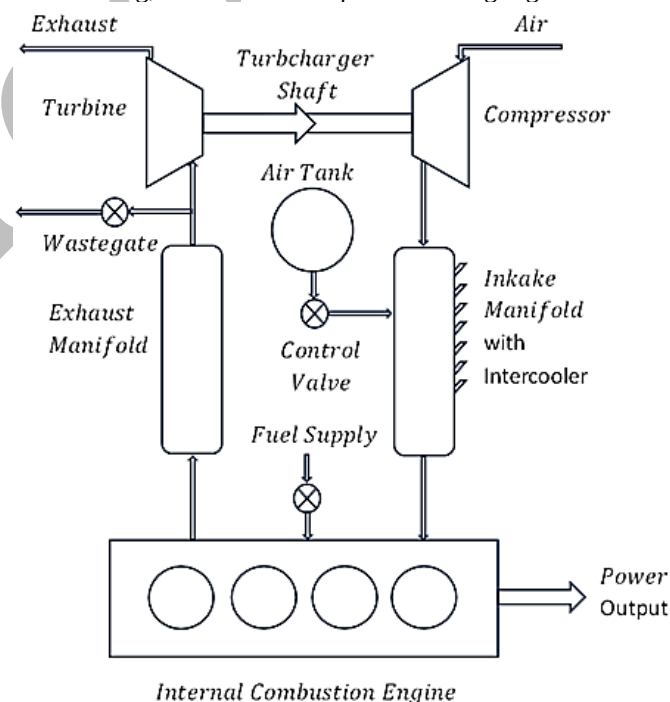
Figure 1. Schematic representation of the system modeling components
