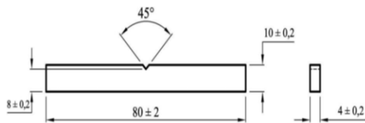
Figure 3. (a) Specimen dimension for Ogoshi wear test and hardness test, (b) Ogoshi wear test and hardness test specimen
