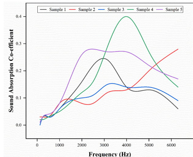
Figure 13. Sound absorption coefficient of various samples
