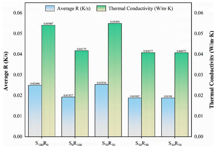
Figure 5. Thermal properties of hybrid polymer composite
