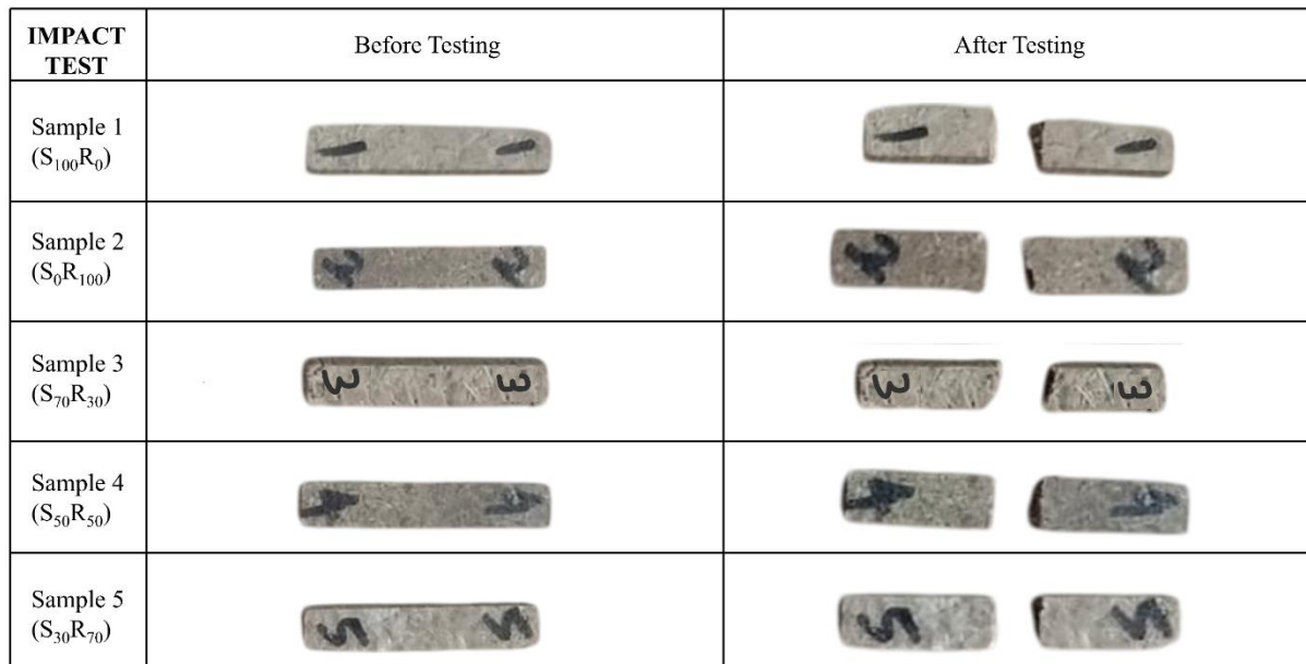
Figure 11. Before and after testing images of the impact test samples
