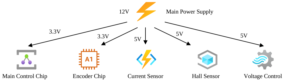
Figure 2. Legend of voltage supply for motor conversion
