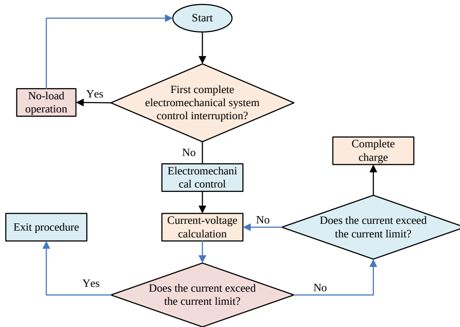
Figure 4. Interrupt control process of electromechanical servo system
