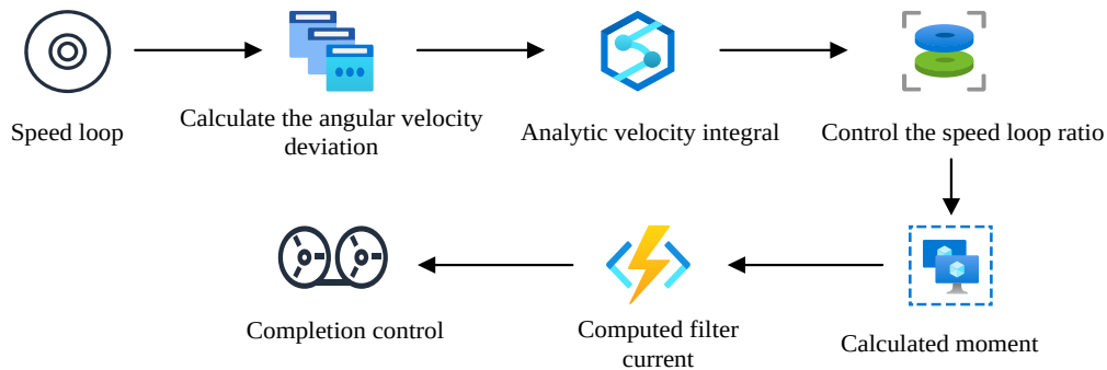
Figure 5. Motor speed control process
