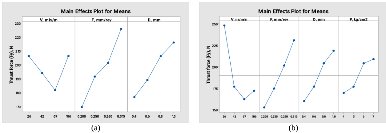
Figure 8. Optimization plots for thrust force ( F_y ) using uncoated tools for (a) Dry machining, and (b) MQL machining
