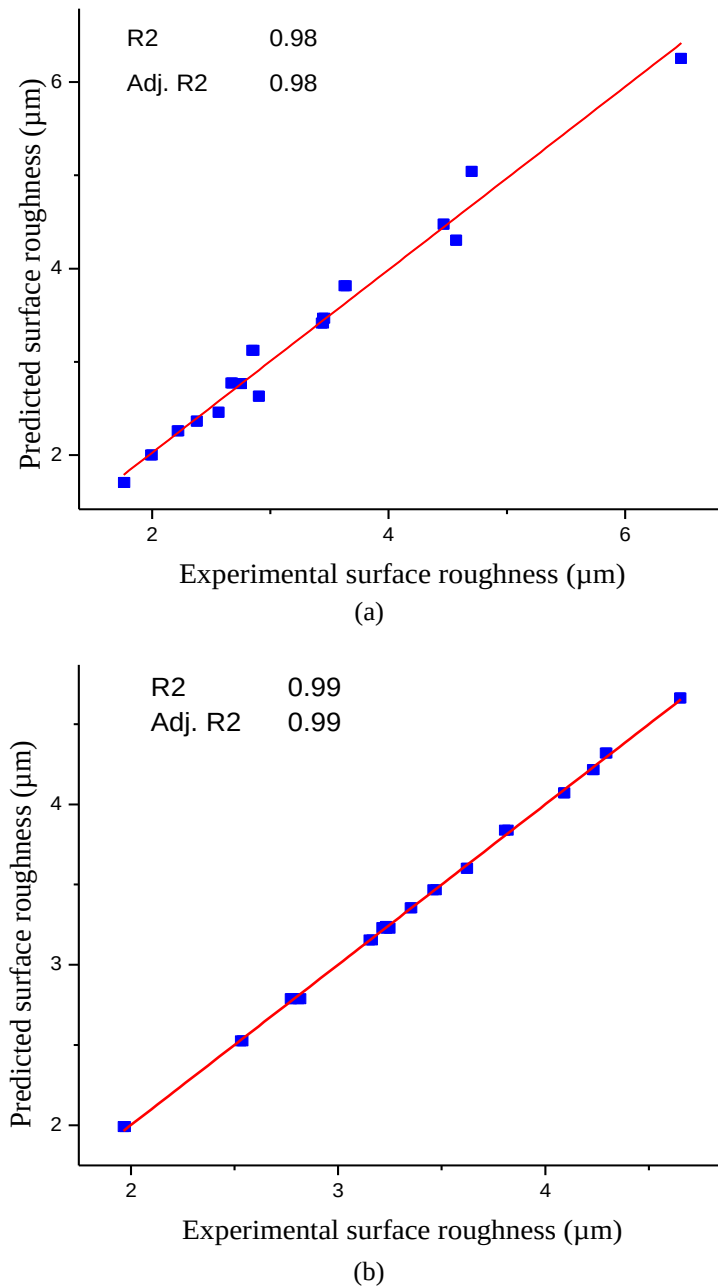
Figure 14. Experimental results vs predicted results with PVD coated tools for surface roughness for (a) Dry machining, and (b) MQL machining
