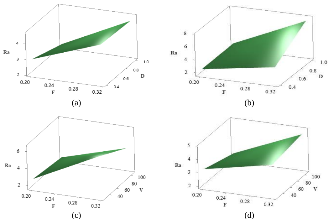
Figure 10. Surface plots for major influence parameters as combined effects on surface roughness for (a) Dry turning with uncoated tool, (b) MQL turning using uncoated tool, (c) Dry turning using PVD coated tool, and (d) MQL turning using PVD coated tool
