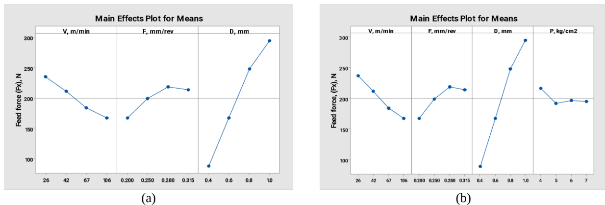
Figure 7. Optimization plots for feed force (Fx) using PVD coated tools for (a) Dry machining, and (b) MQL machining
