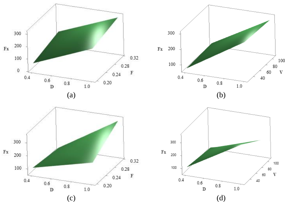
Figure 12. Surface plots for major influence parameters as combined effects on feed force for (a) Dry turning with uncoated tool, (b) MQL turning using uncoated tool, (c) Dry turning using PVD coated tool, and (d) MQL turning using PVD coated tool
