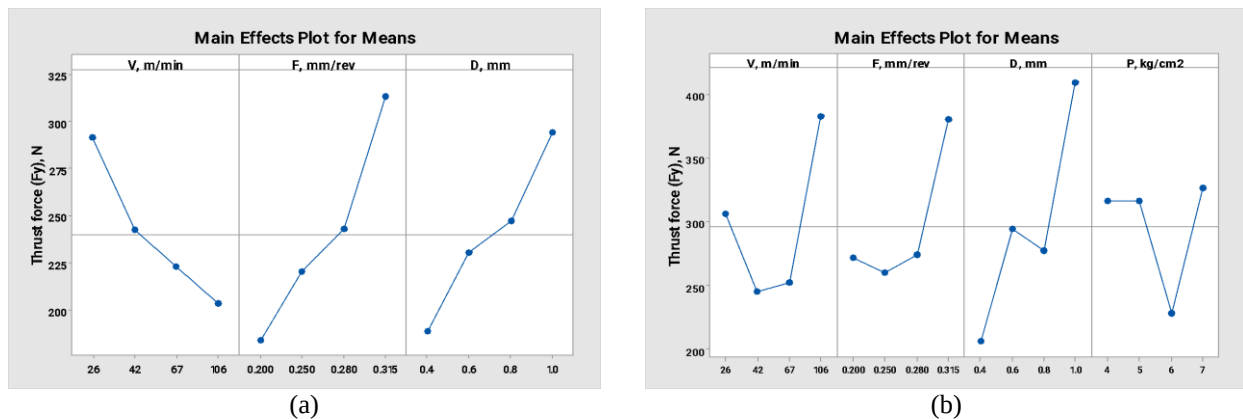
Figure 9. Optimization plots for thrust force ( F_y ) with PVD coated tools for (a) Dry machining, and (b) MQL machining
