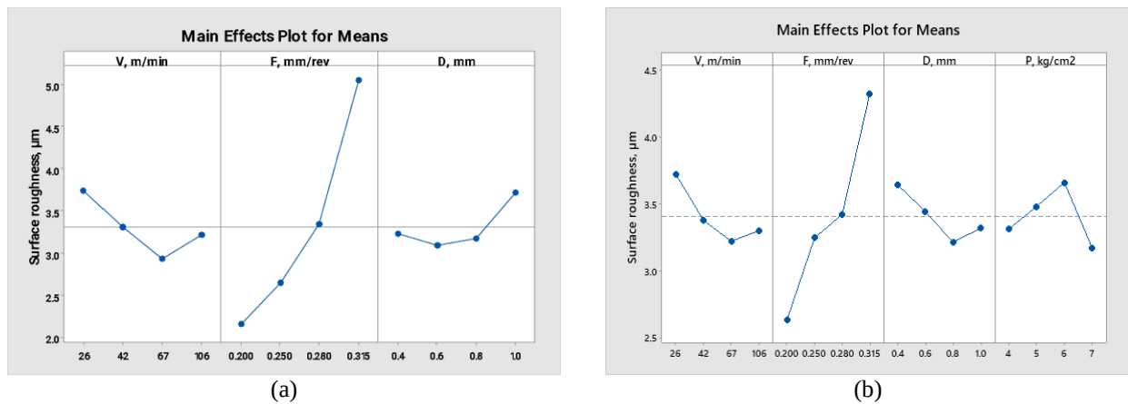
Figure 3. Optimization plots using PVD coated tools for surface roughness for (a) Dry machining, and (b) MQL machining
