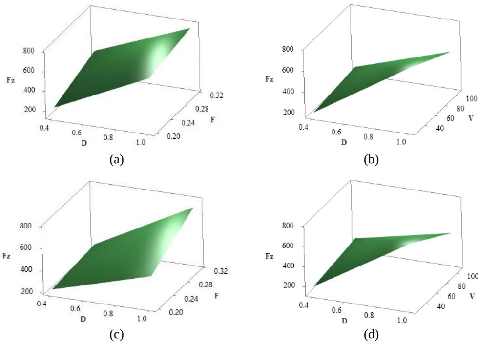
Figure 11. Surface plots for major influence parameters as combined effects on cutting force for (a) Dry turning with uncoated tool, (b) MQL turning using uncoated tool, (c) Dry turning using PVD coated tool, and (d) MQL turning using PVD coated tool
