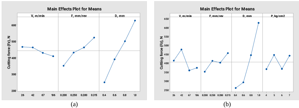
Figure 5. Optimization plots for cutting force ( F_z ) using PVD coated tools for (a) Dry machining, and (b) MQL machining
