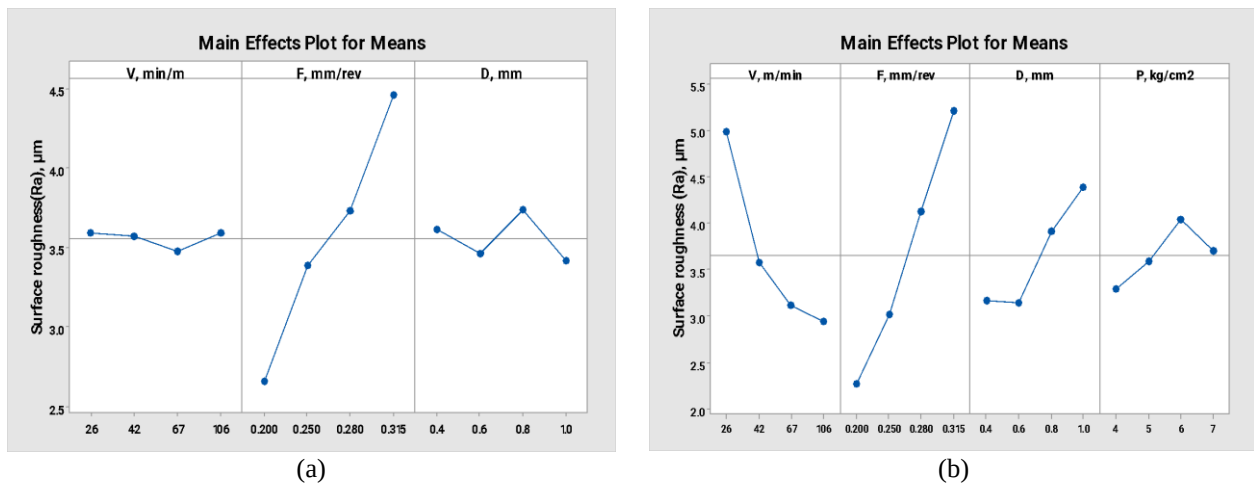
Figure 2. Optimization plots using uncoated tools for surface roughness for (a) Dry machining, and (b) MQL machining
