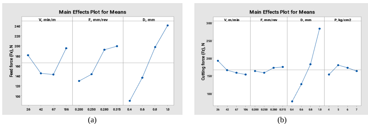
Figure 6. Optimization plots for feed force ( F_x ) using uncoated tools for (a) Dry machining, and (b) MQL machining
