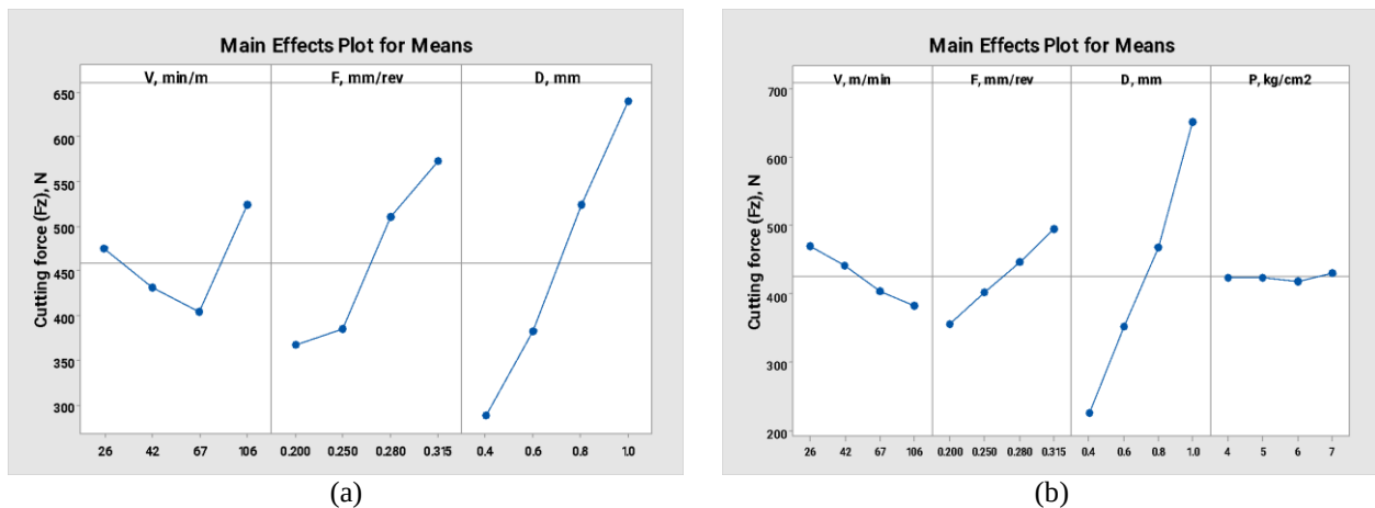
Figure 4. Optimization plots for cutting force (Fz) using uncoated tools for (a) dry machining, and (b) MQL machining
