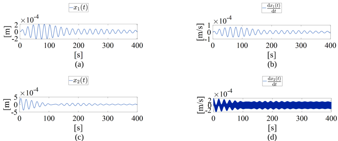
Figure 8. Transient simulation results of the 2-DoF system in mechanical coordinates. Initial conditions x_{i0}(t) = \frac{dx_{i0}(t)}{dt} = 0 where i \in \{1, 2\} . (a) Dynamics of x_1(t) . (b) Dynamics of \frac{dx_1(t)}{dt} . (c) Dynamics of x_2(t) . (d) Dynamics of \frac{dx_2(t)}{dt}
