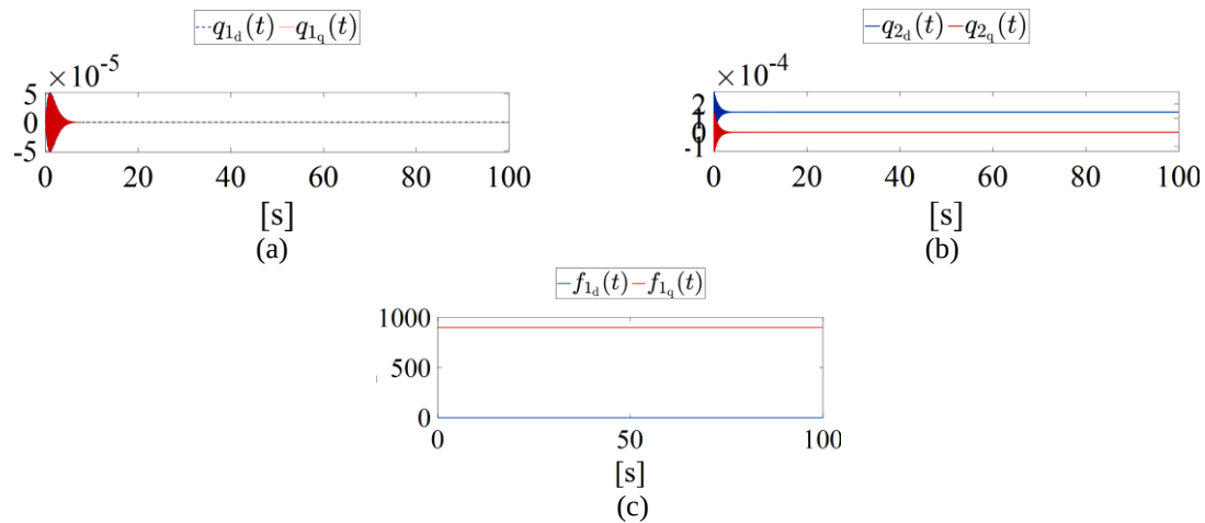
Figure 7. Transient simulation results of the 1-DoF system in dq coordinates. Initial conditions q_{mn}(t) = 0 where m \in \{1, 2\} and n \in \{d, q\} . (a) Dynamics of q_{1d}(t) and q_{1q}(t) . (b) Dynamics of q_{2d}(t) and q_{2q}(t) . (c) Dynamics of f_{1d}(t) and f_{1q}(t)
