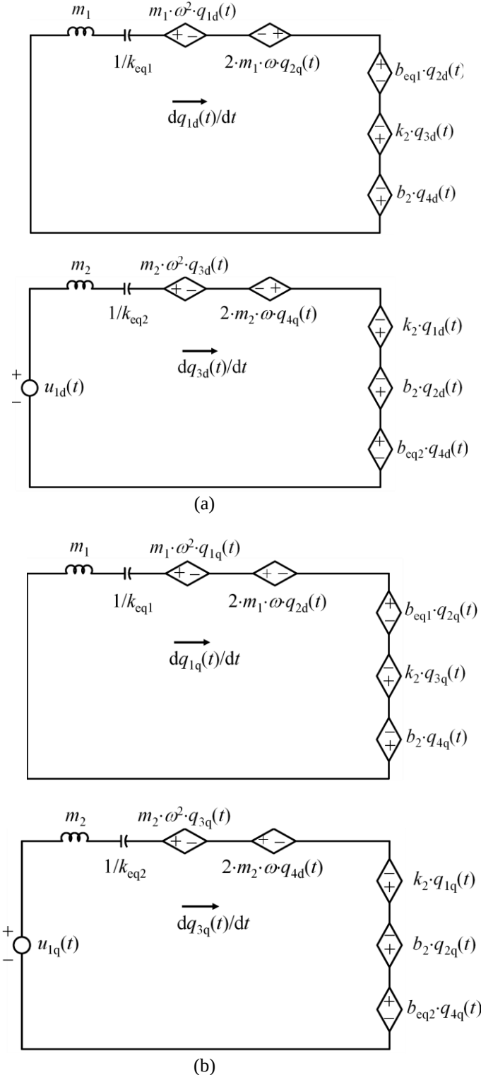
Figure 4. Electrical analogy of the proposed 2-DoF mechanical system in dq coordinates. The two channels d and q are shown (a) Channel d; (b) Channel q
