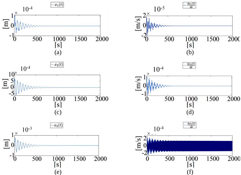
Figure 10. Transient simulation results of the 3-DoF system in mechanical coordinates. Initial conditions x_{i0}(t) = dx_{i0}(t)/dt = 0 for i \in \{1, 2, 3\} (a) Dynamics of x_1(t) ; (b) Dynamics of dx_1(t)/dt ; (c) Dynamics of x_2(t) ; (d) Dynamics of dx_2(t)/dt ; (e) Dynamics of x_3(t) ; (f) Dynamics of dx_3(t)/dt
