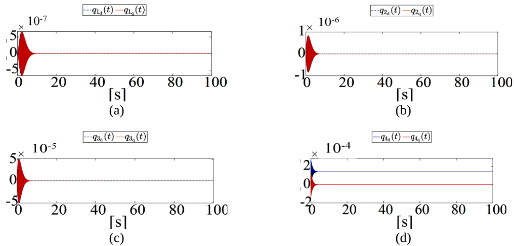
Figure 9. Transient simulation results of the 2-DoF system in dq coordinates. Initial conditions q_{mn}(t) = 0 where m \in \{1, 2, 3, 4\} and n \in \{d, q\} . (a) Dynamics of q_{1d}(t) and q_{1q}(t) . (b) Dynamics of q_{2d}(t) and q_{2q}(t) . (c) Dynamics of q_{3d}(t) and q_{3q}(t) . (d) Dynamics of q_{4d}(t) and q_{4q}(t)
