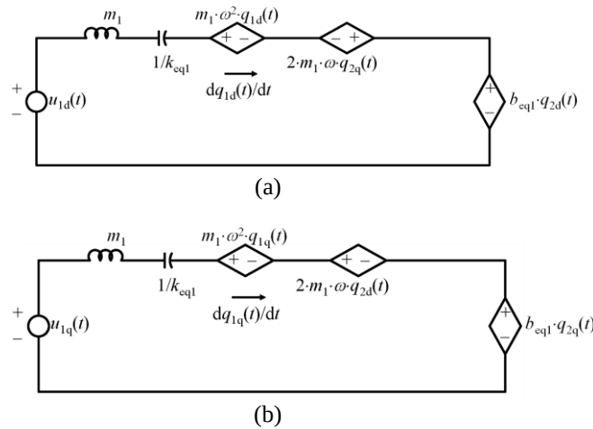
Figure 3. Electrical analogy of the proposed 1-DoF mechanical system in dq coordinates. The two channels d and q are shown (a) Channel d; (b) Channel q
