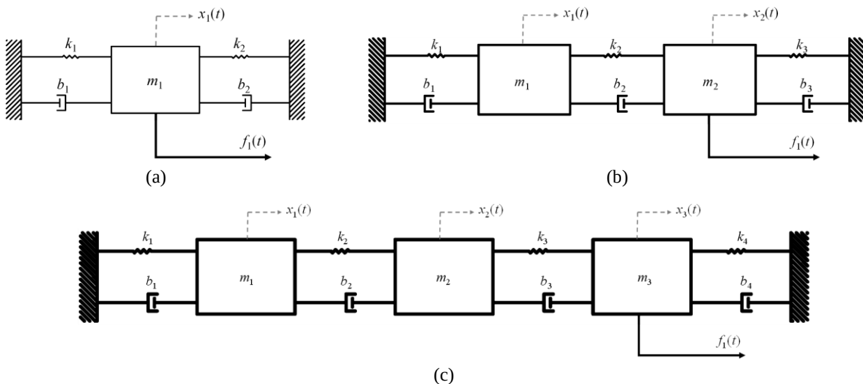
Figure 2. Proposed vibrational mechanical dynamic models to which dq0 will be applied (a) 1-DoF; (b) 2-DoF; (c) 3-DoF
