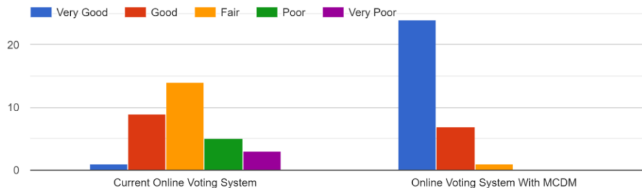
Figure 9 Compariosn Usability Between Current Online Voting System and Online Voting System with MCDM method
