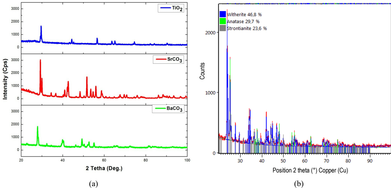
Figure 1. X-ray diffraction patterns of TiO 2 , SrCO 3 and BaCO 3 powders (a) before and (b) after 58 hours of milling.
