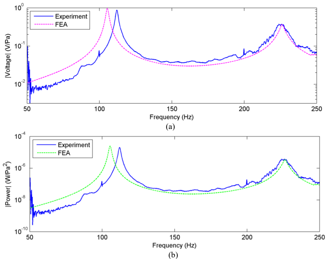
Figure 10. Frequency response at optimum resistive load for experiment and FEA: (a) voltage with load resistance ( VL/p_1 ) (b) power output ( Power/p_1^2 )
