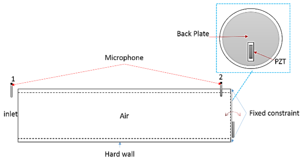
Figure 4. Acoustic structure piezoelectric interaction boundary requirement for AEHs
