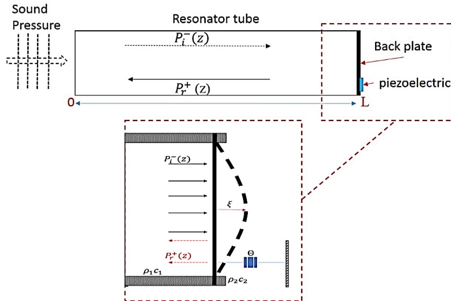
Figure 1. A quarter-wavelength resonator tube's L length experienced a sound pressure reflected at the flexible backplate
