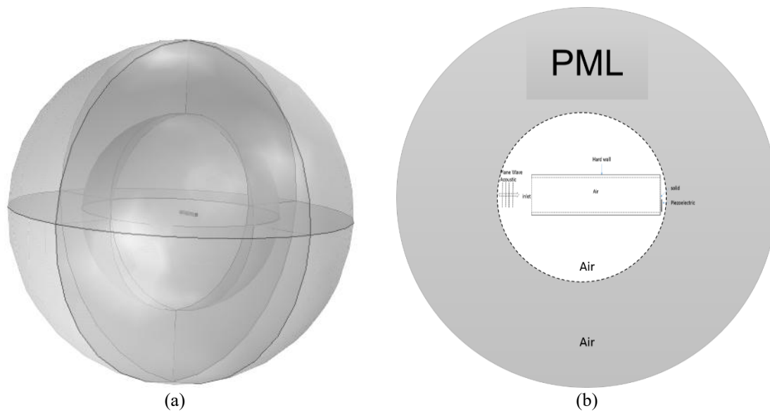
Figure 3. Fully connected finite model element: (a) a three-dimensional model comprising a quarter-wavelength resonator, plane wave source domain, and PML domain (b) a 2D model that depicts a 3D model part
