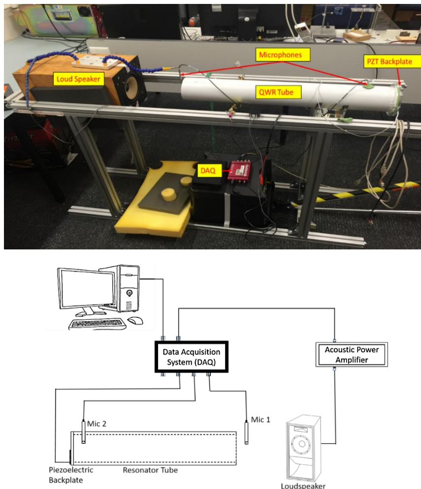
Figure 6. A quarter-wavelength resonator and a flexible PZT backplate are used in the experimental setup and schematic diagram for acoustic energy collection
