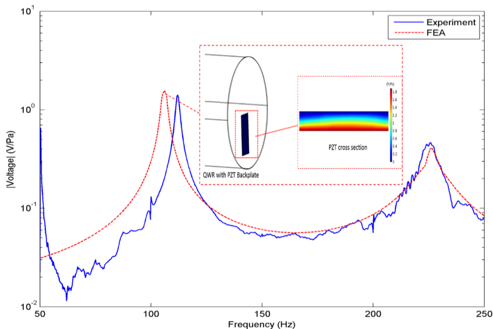
Figure 8. Frequency response of (OCV/p_1) for experiment and FEA. Small figure FEA 3-D plot
