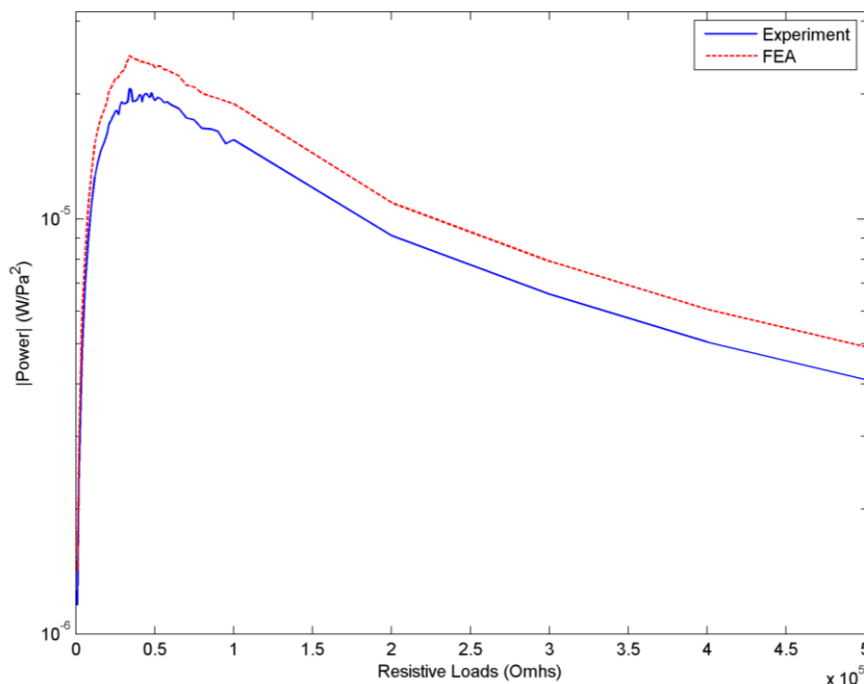
Figure 9. Experiment and FEA results for the output power of the AEHs for different resistive loads
