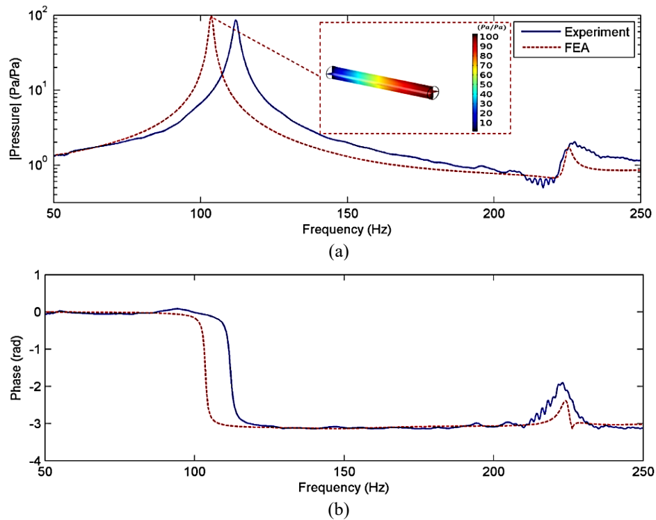
Figure 7. Acoustic pressure ratio ( p_2/p_1 ) frequency response for experiment and FEA: (a) Magnitude and a small figure is a 3-D plot from FEA (b) phase
