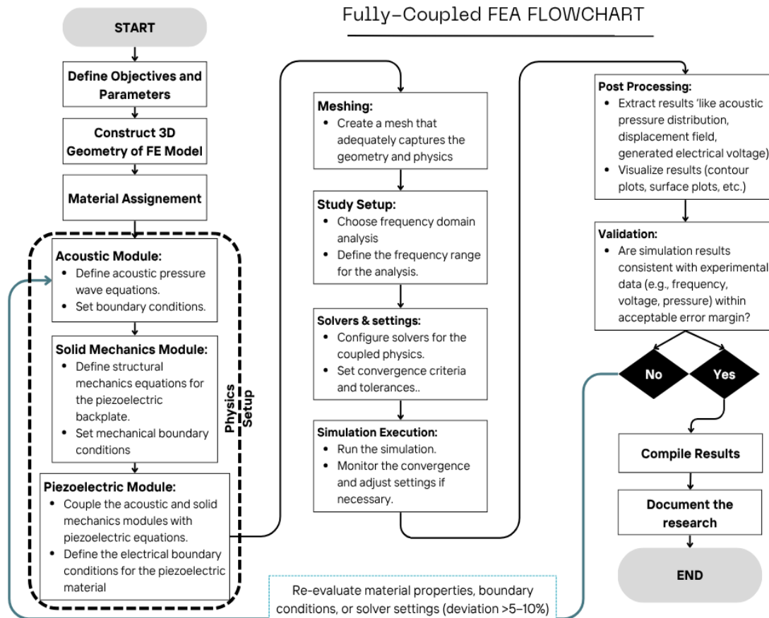
Figure 2. Fully-coupled finite element analysis, Multiphysics AEH system flowchart
