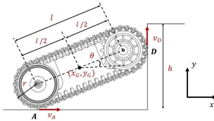
Figure 2. Kinematics of step climbing
