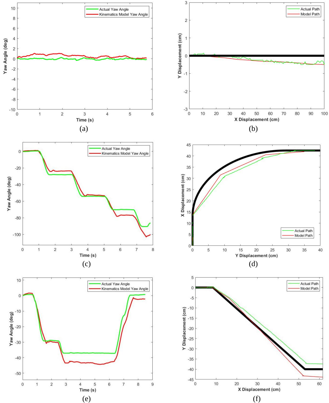
Figure 13. Yaw angle and position result (a)(b) Straight-line course, (c)(d) radius curve course and (e)(f) sharp curve course
