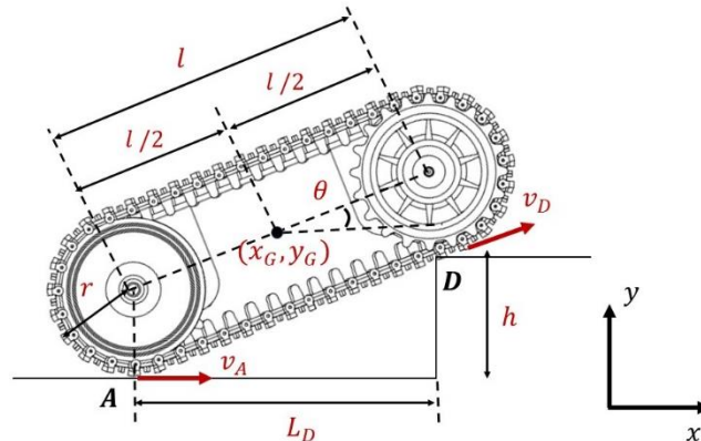
Figure 4. Kinematics model of step crossing
