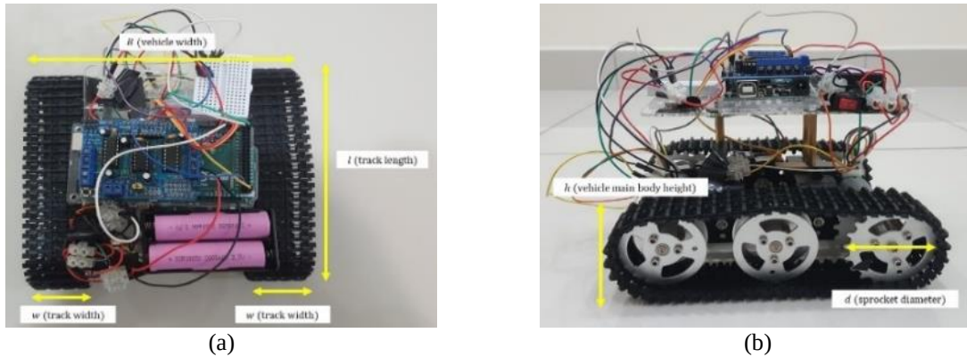
Figure 5. Platform of TP100 crawler: (a) view from the top (b) view from the side
