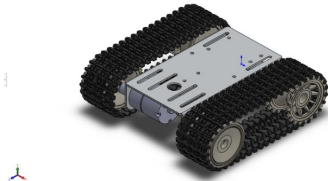
Figure 6. The SolidWorks® CAD model of the TP100 crawler caterpillar
