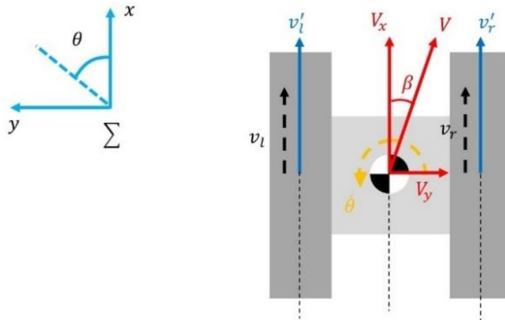
Figure 1. Kinematics model of tracked car
