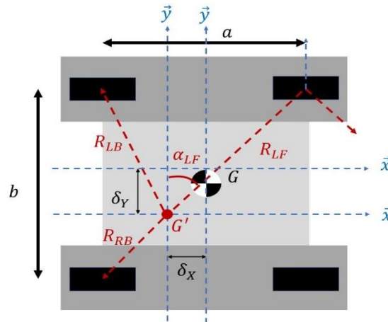
Figure 8. Schematic of skid-steered tracked car
