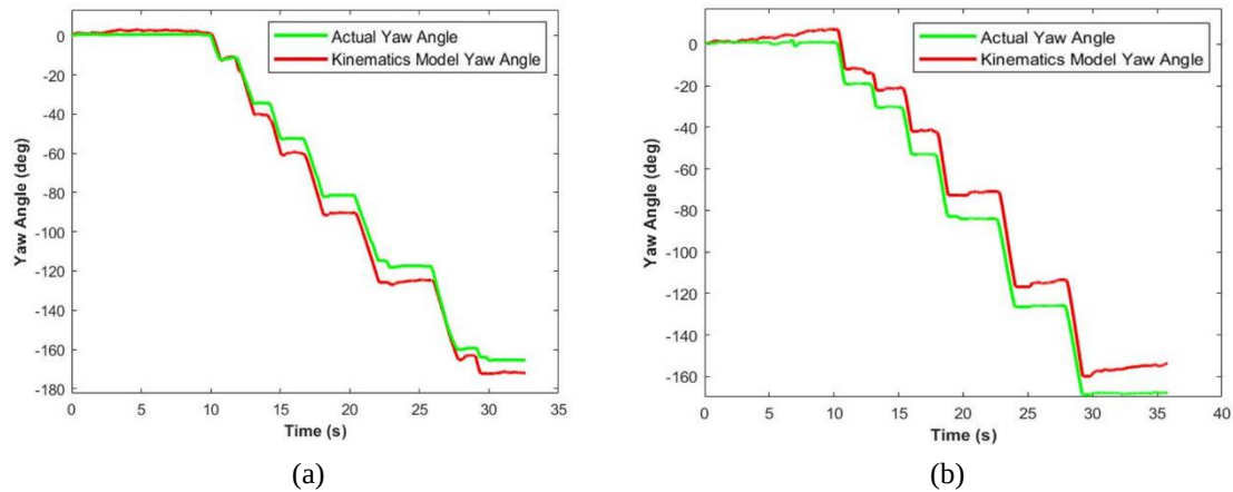
Figure 17. Trajectory tracking control - yaw angle (a) behaviour test course 2 and (b) behaviour test course 3
