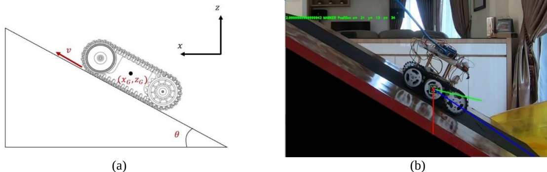
Figure 10. (a) Kinematics model of ramp climbing (b) Experiment of ramp climbing
