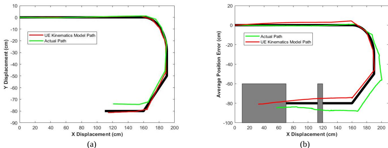
Figure 18. Trajectory tracking control – spatial displacement (a) behaviour test course 2 (b) behaviour test course 3
