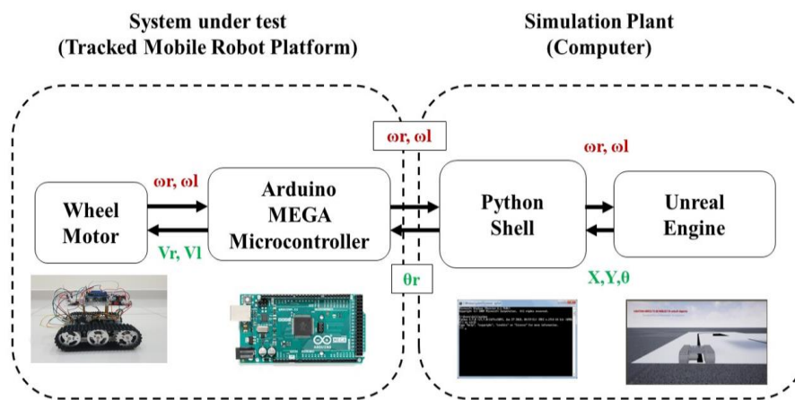
Figure 14. Interactive simulation with Hardware-In-The-Loop
