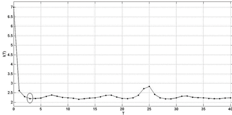
Figure 4. Average mutual information result ( \tau = 3 )
