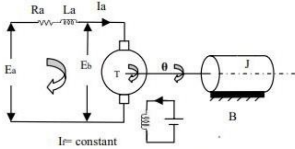
Figure 1. Brushed DC motor circuit
