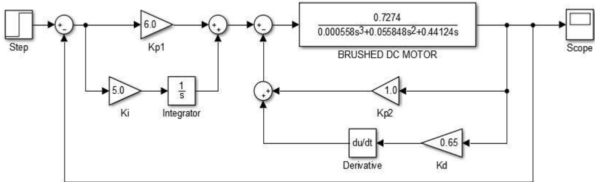
Figure 3. Block diagram of PI-PD controller in MATLAB/Simulink
