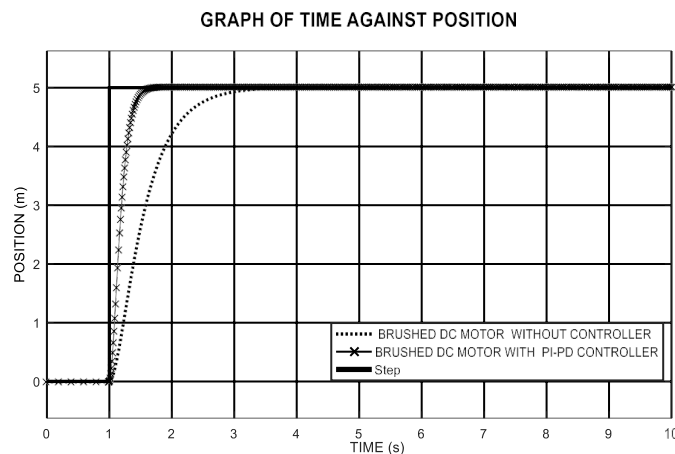
Figure 5. Combination graph of brushed DC motor without controller and brushed DC motor with PI-PD Controller
