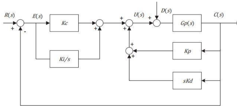
Figure 2. Block diagram of PI-PD controller
